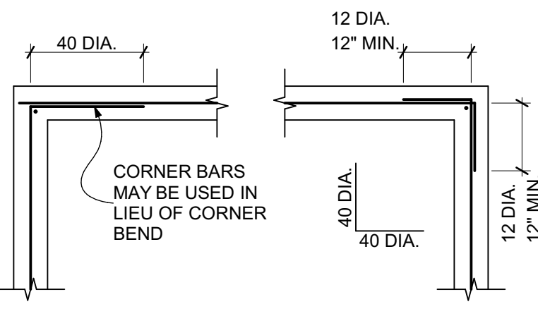
TYP. CORNER REINFORCING SCALE: 1/2" = 1'-0"
