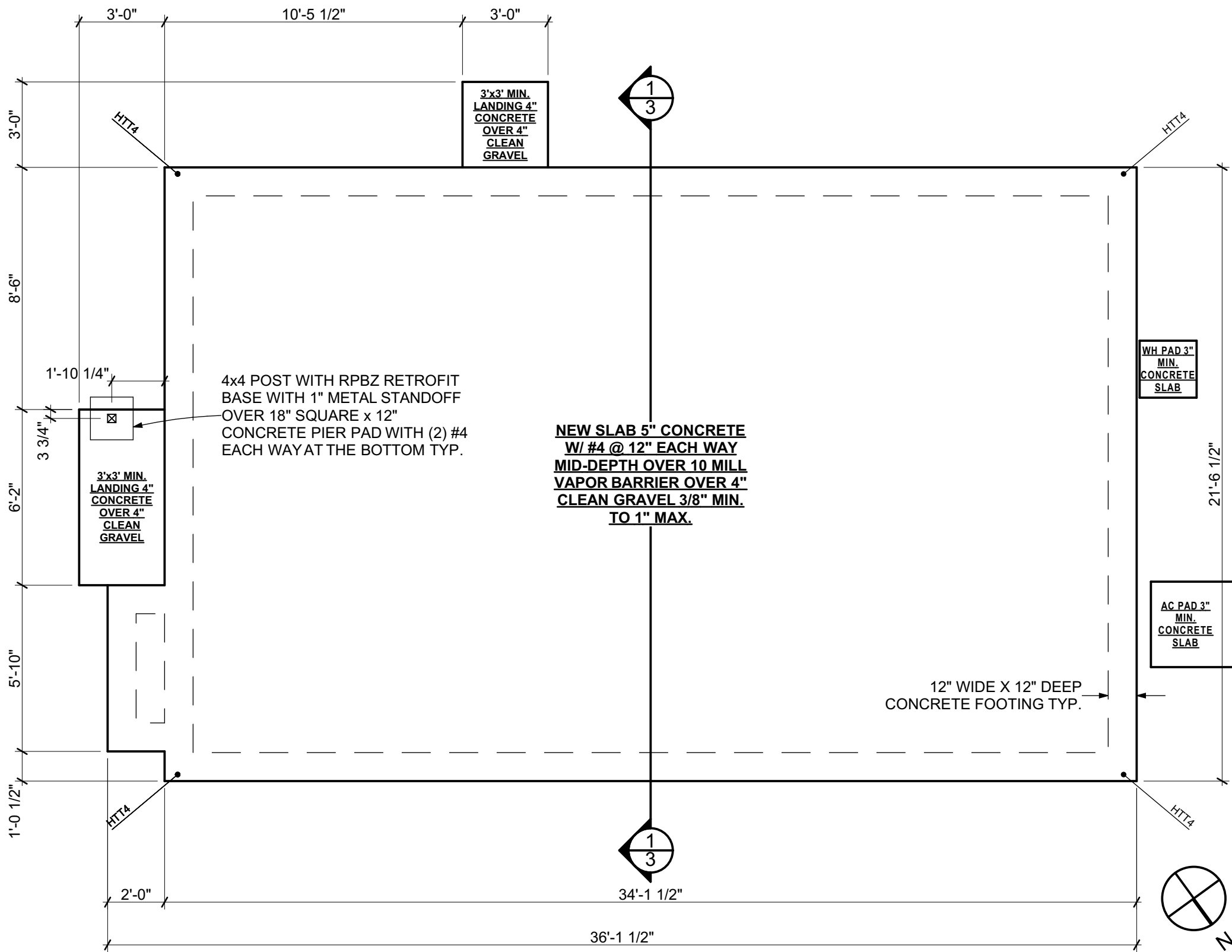
2 FOUNDATION PLAN SCALE: 1/4" = 1'-0"
