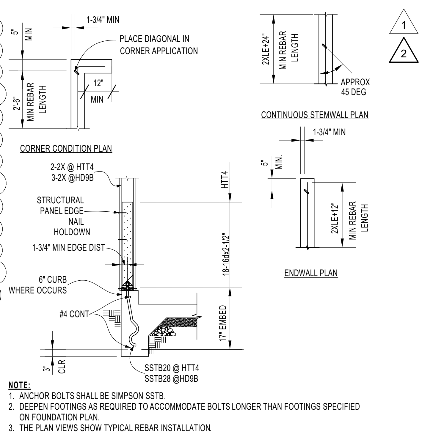
2. HOLDOWN INSTALLATION SCALE: 3/4" = 1'-0"
