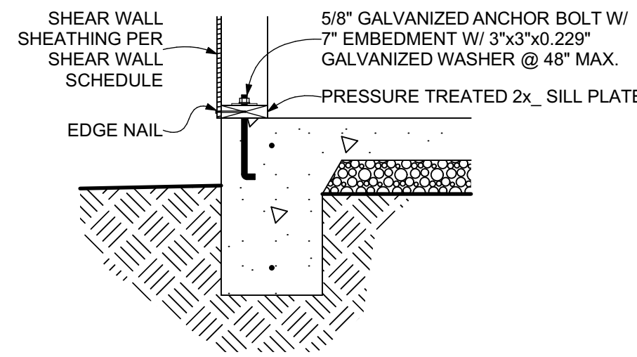
5 SHEAR TRANSFER @ FOUNDATION SCALE: 3/4" = 1'-0"
