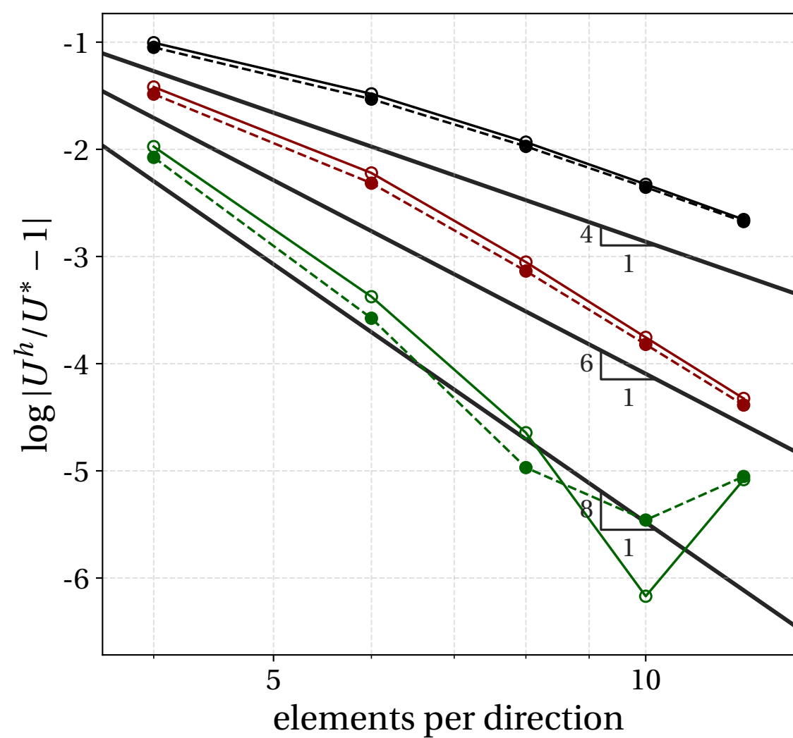
(a) 1/t = 100
