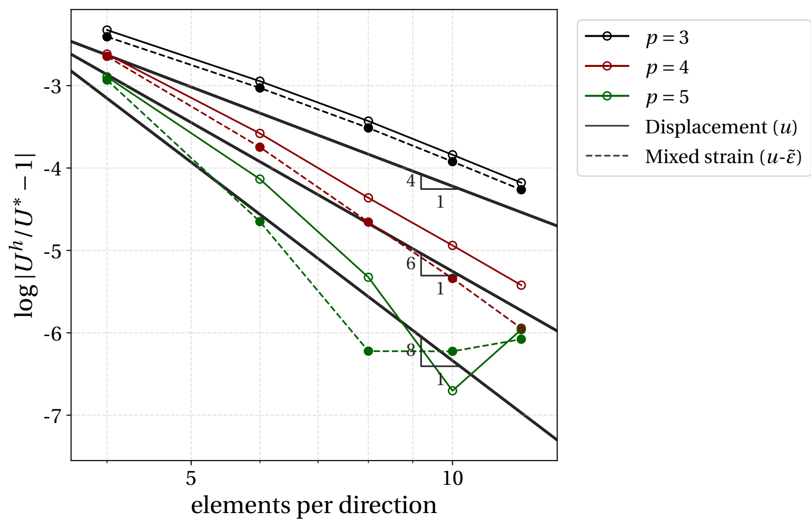
(b) 1/t = 100000
