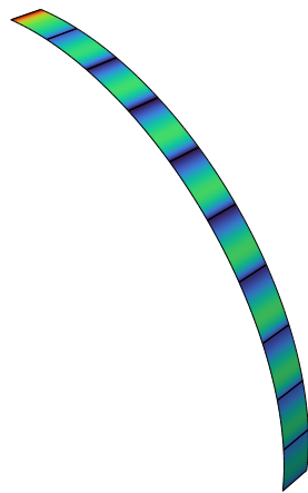
(c) RM-4p, R/t = 10000
