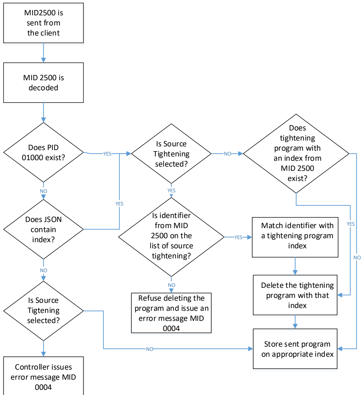
Figure 3: The program flow
