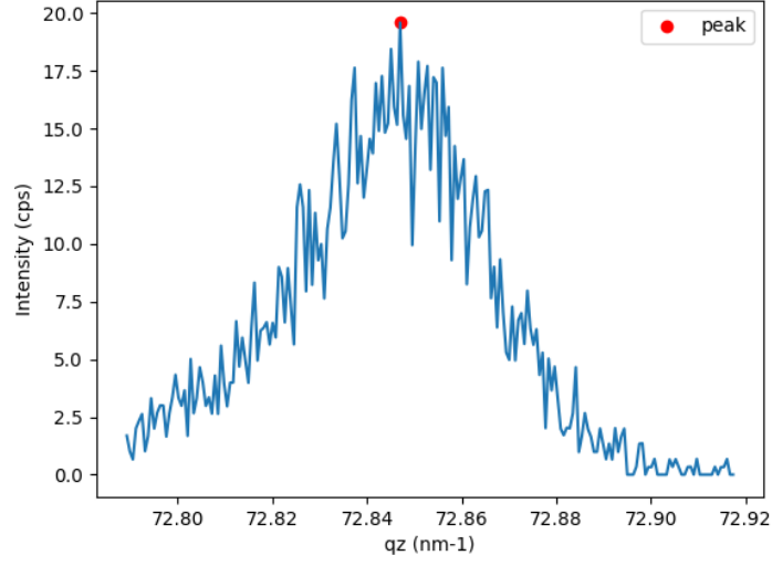
Figure 8: 2\theta/\omega scan of sample C (006) in unit of q_{\perp}
