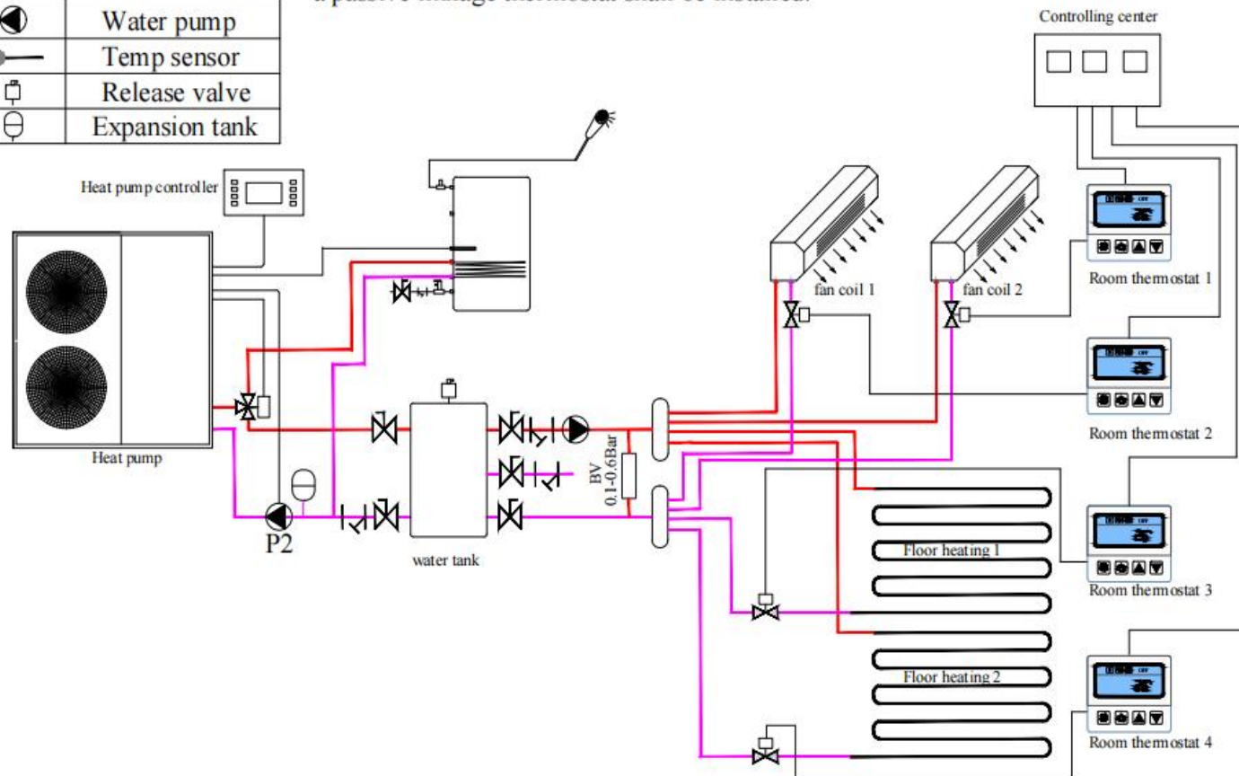
DC inverter air source heat pump
