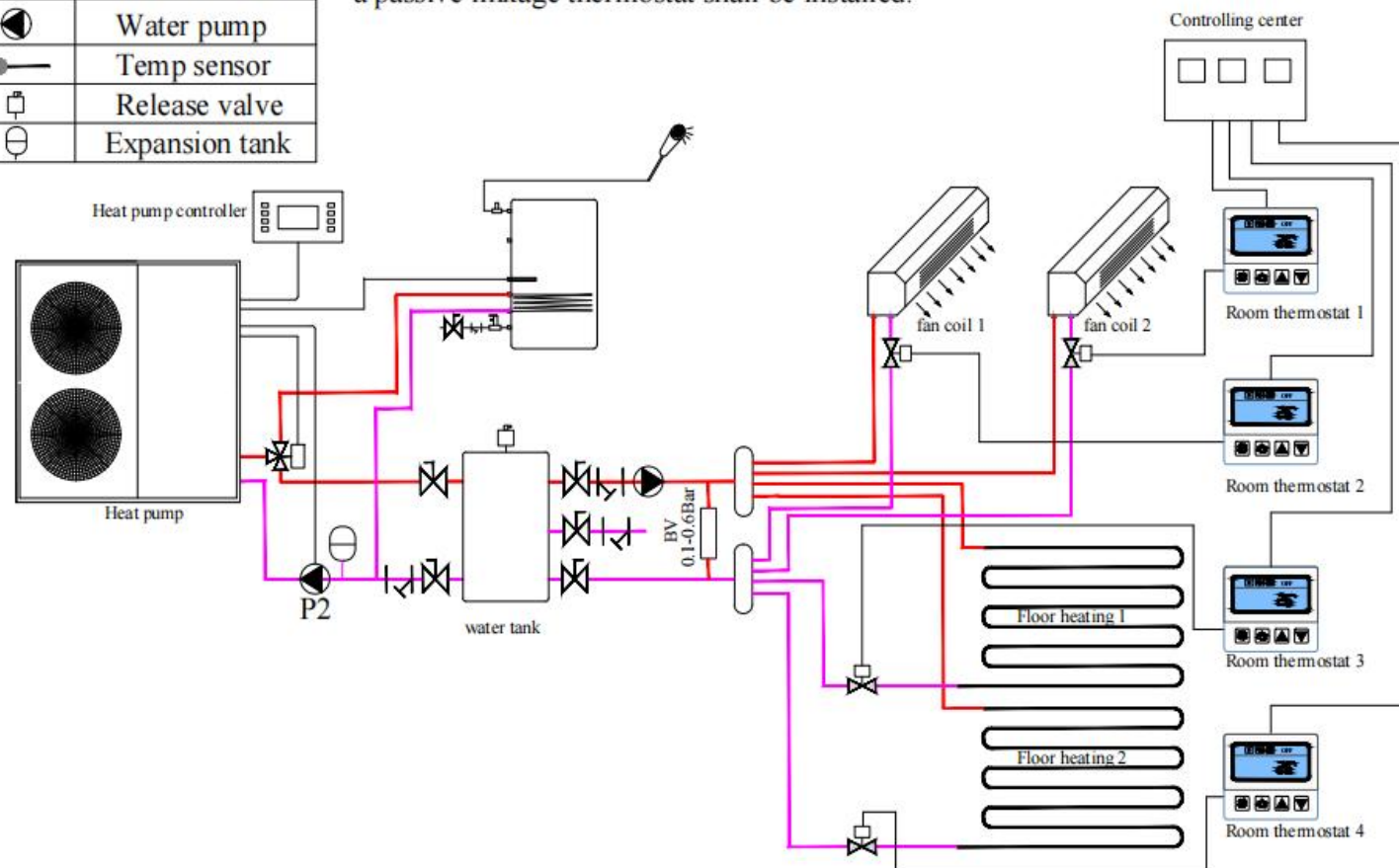
DC inverter air source heat pump
