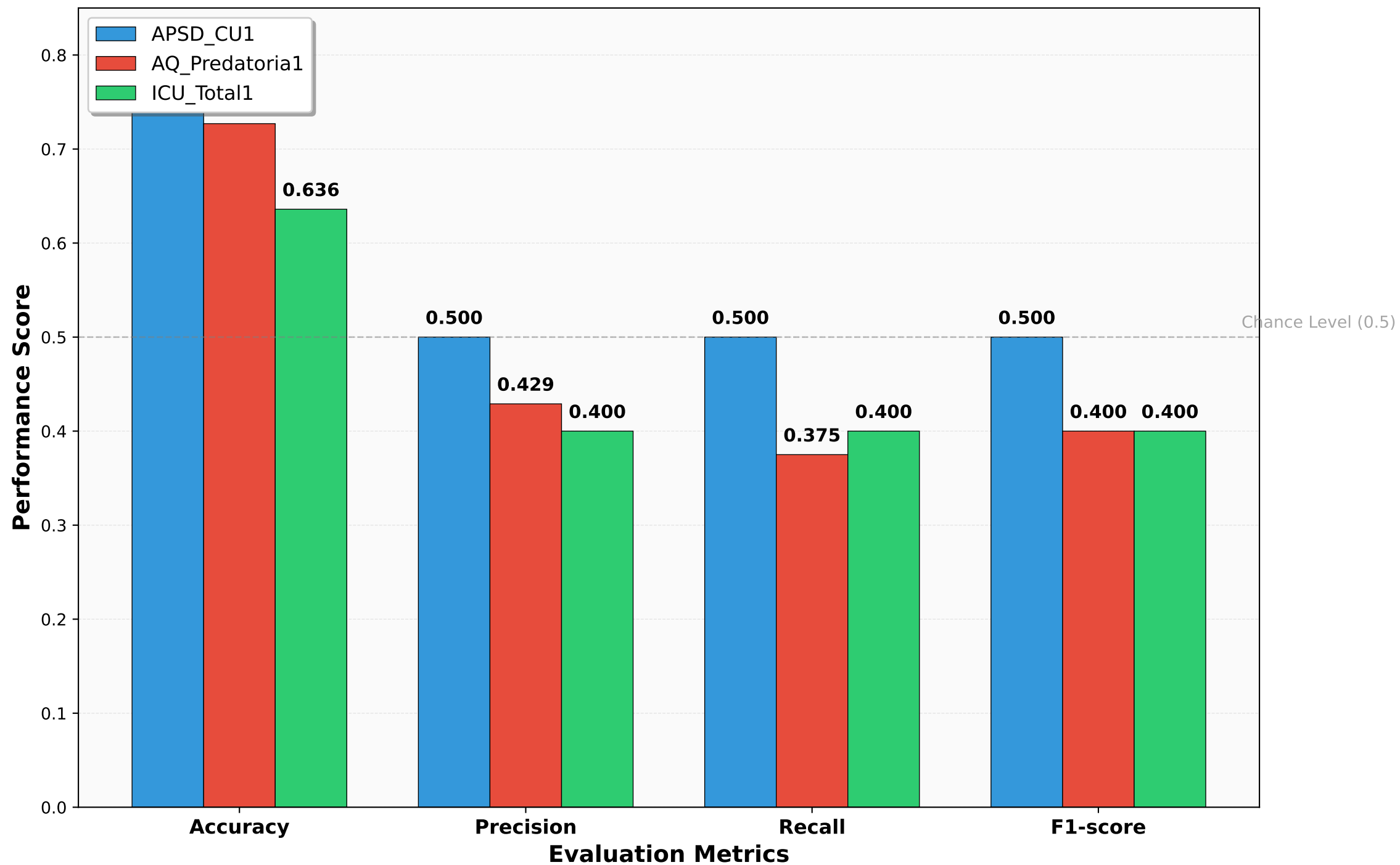
Model Performance Comparison Across Outcomes
