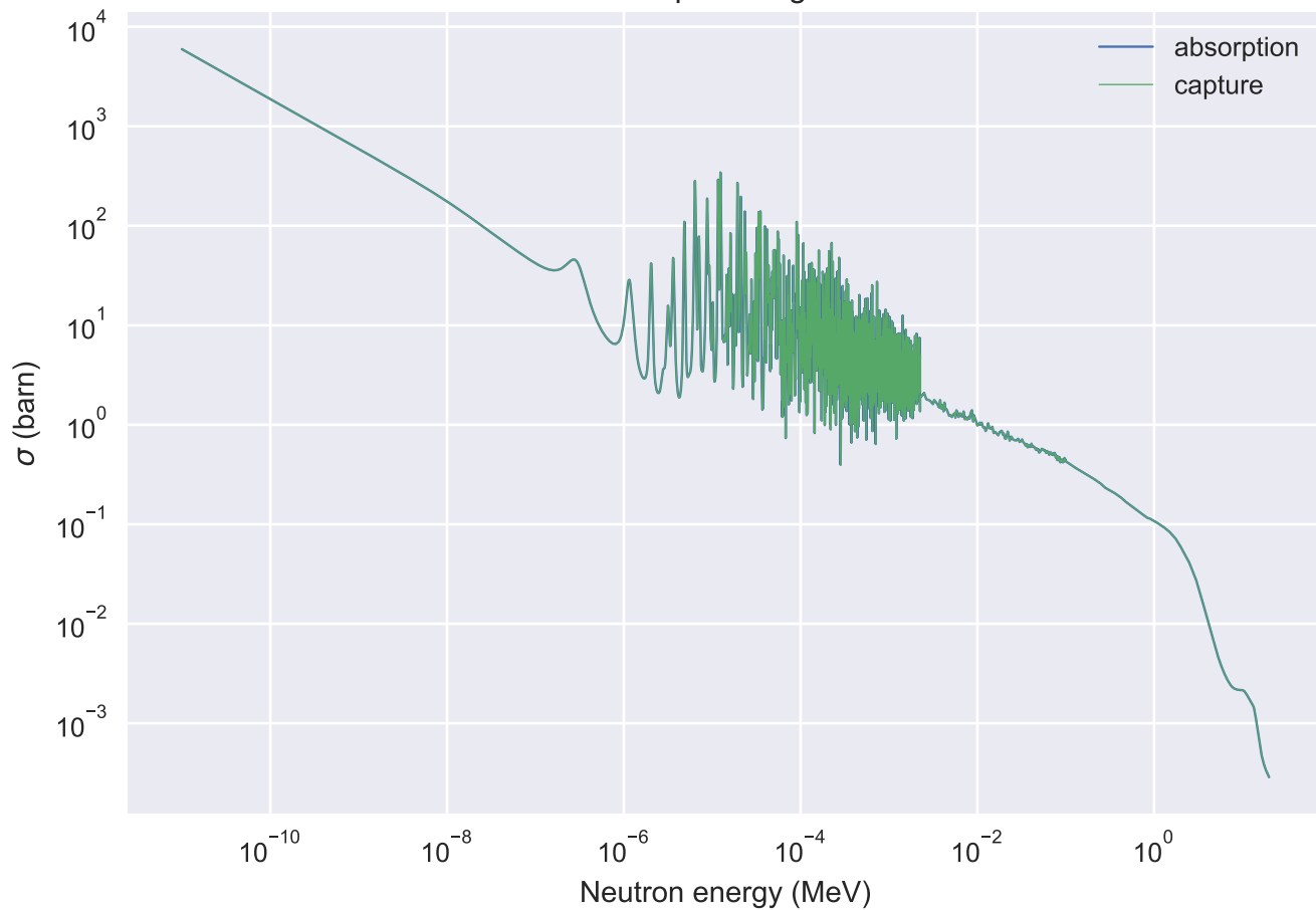
U-235 absorption bug at 1200 K
