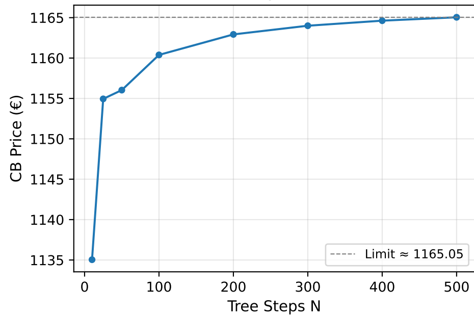
Tree Convergence — Price
