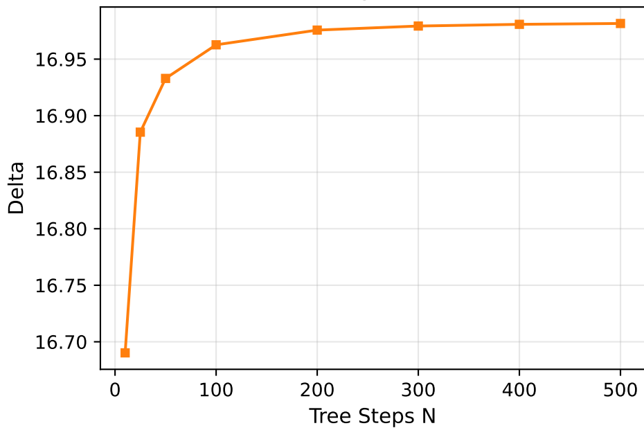
Tree Convergence — Delta
