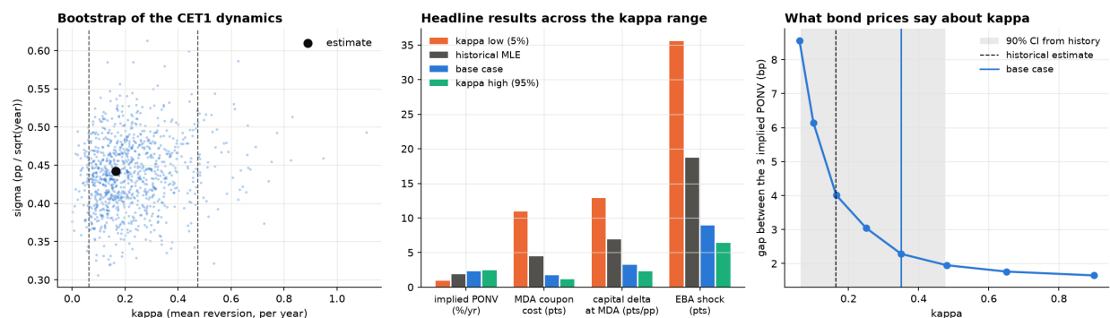
Figure 3: Left: bootstrap of (\kappa, \sigma) . Centre: headline results across the \kappa range. Right: cross-bond dispersion of the implied hazard against \kappa .
