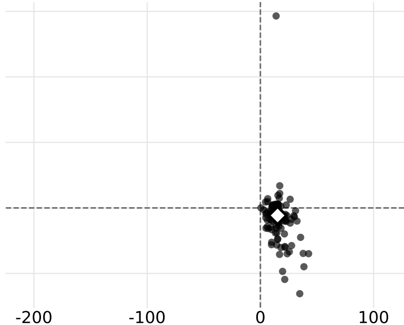
DS19 + IF2 warm start (J=1,000)
