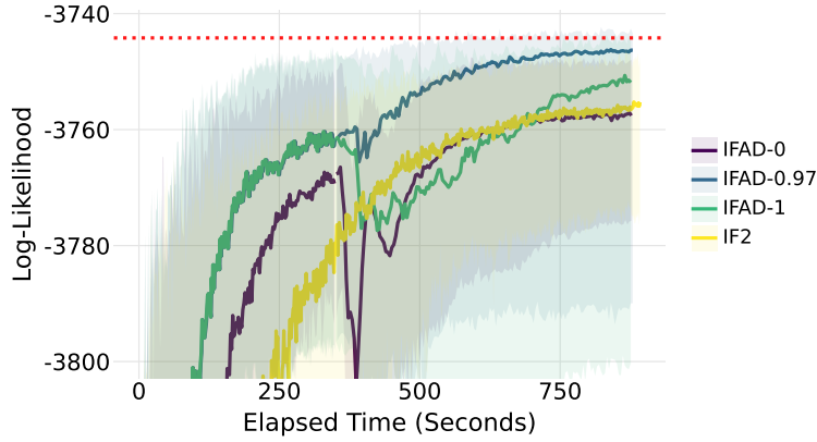
Figure 5: Optimization progress of IFAD and IF2. The shaded regions cover the area between the 100th and 10th percentiles of log-likelihood estimates at each iteration. We use a dotted red line to display the MLE.
