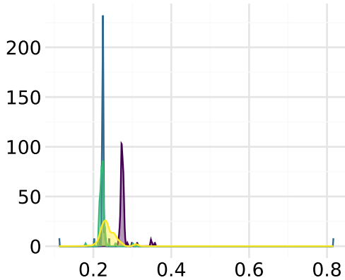
Measurement noise ( \tau )
