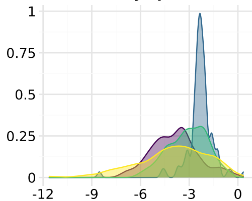
Seasonality spline (bs3)
