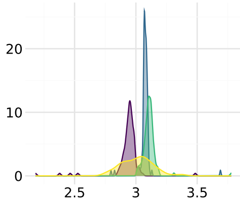
Process noise ( \sigma )
