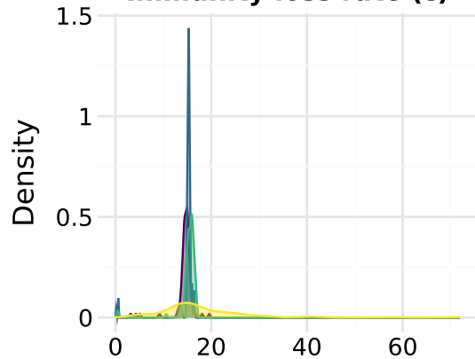
Immunity loss rate ( \epsilon )
