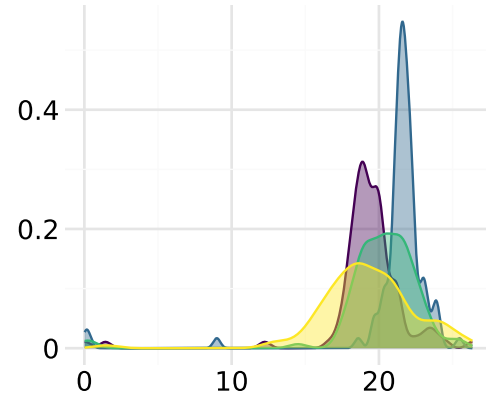
Recovery rate ( \gamma )
