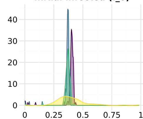
Initial infected ( I_0 )
