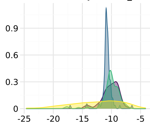
Reservoir spline ( \omega_5 )
