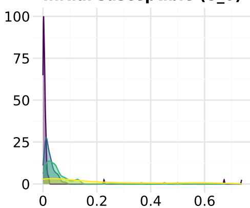
Initial susceptible ( S_0 )
