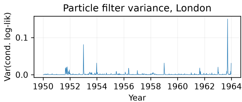
Figure 7: Variance of conditional log-likelihoods across replicates. Observations with high variance are numerically problematic.
