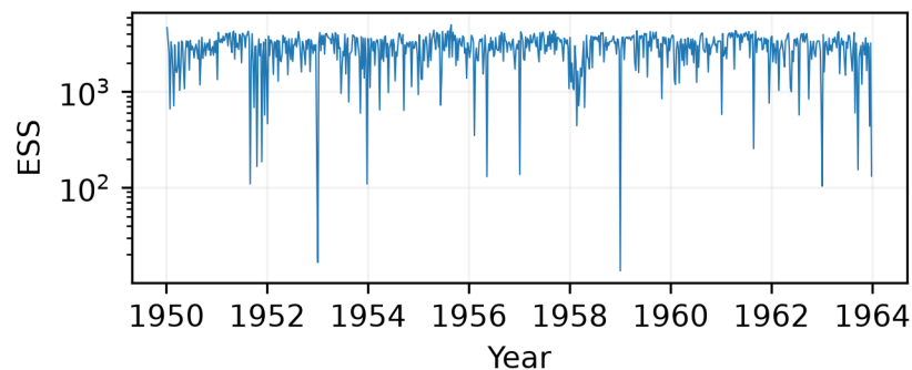
Figure 9: Mean of replicated ESS.
