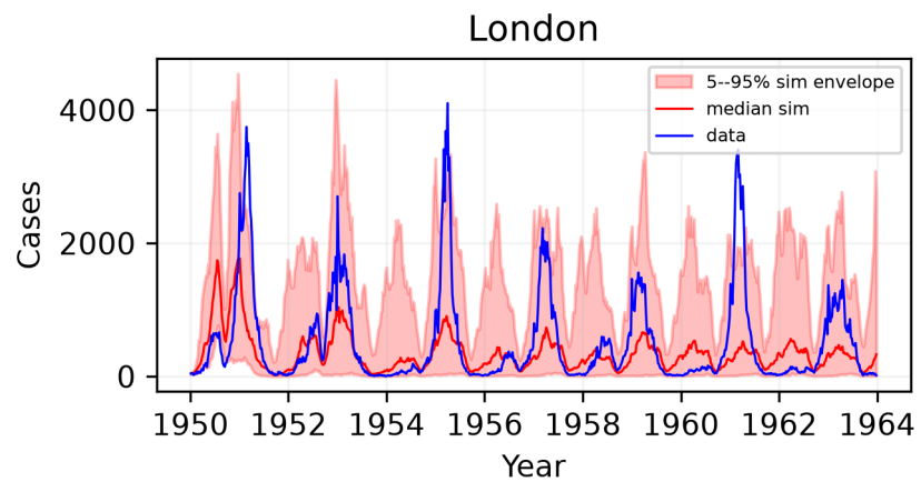
Figure 5: Simulation envelope (100 sims) versus data.
