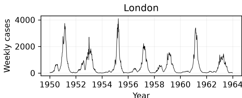
Figure 2: Weekly measles case reports, London 1950–1963.
