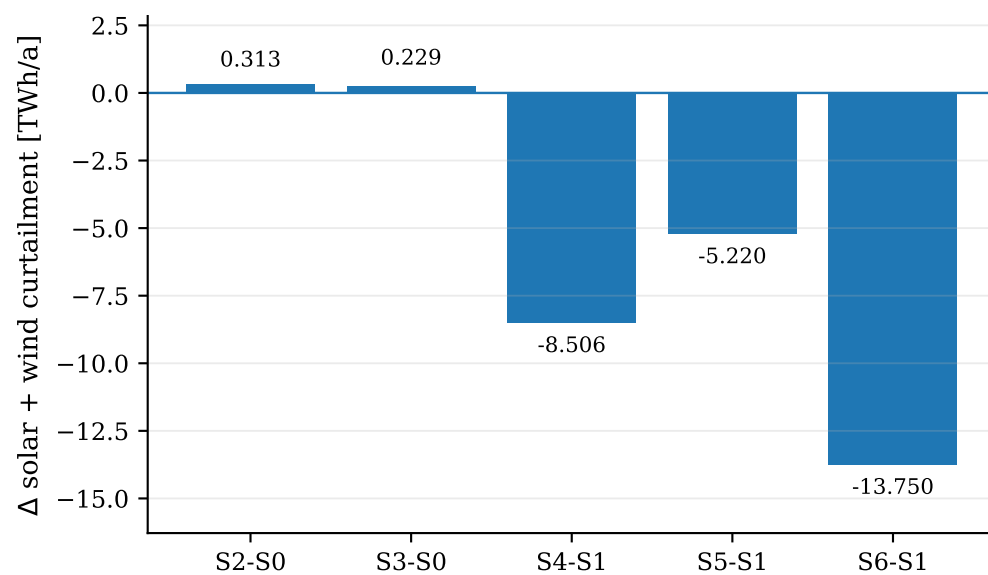
Variable-renewable curtailment
