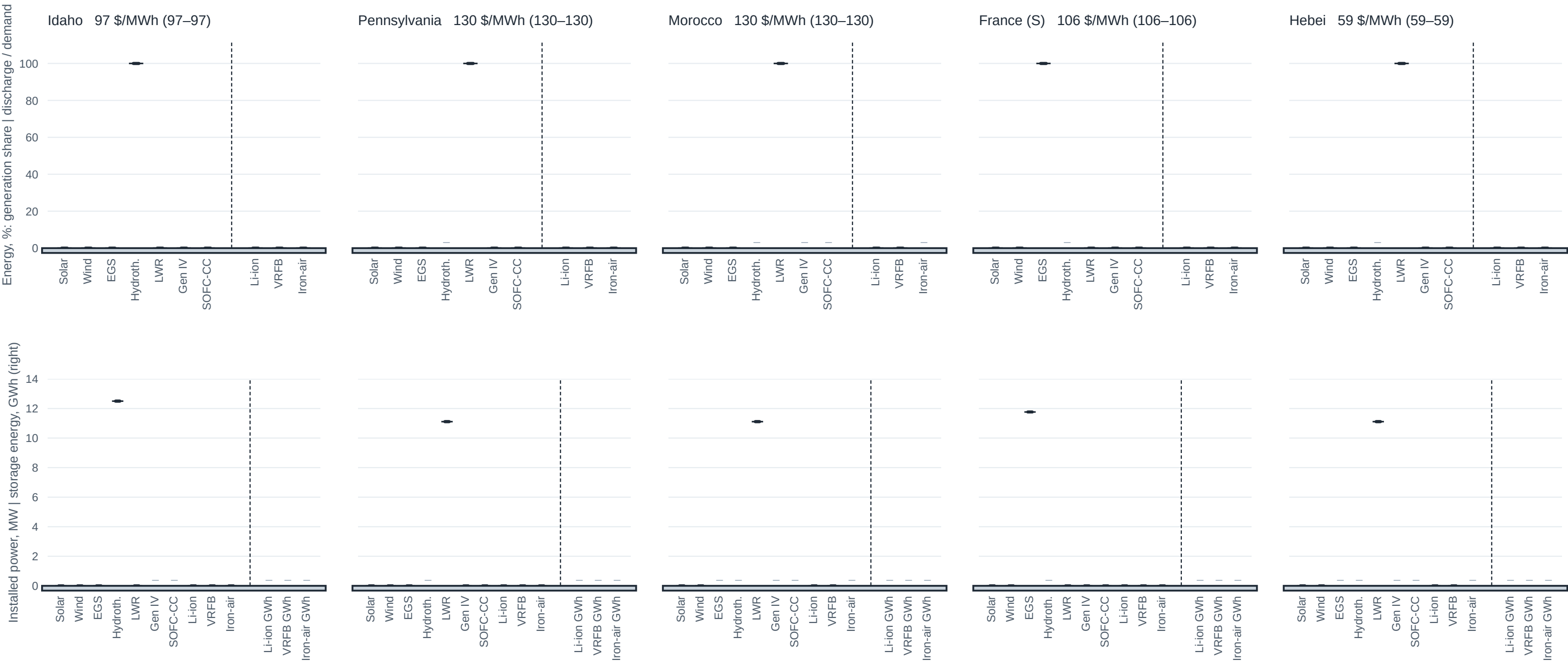
A constant 10 MW supplied 100 % clean in isolation, per site and weather year (10 years): technology_assumptions.csv, 7 % real, no imports
