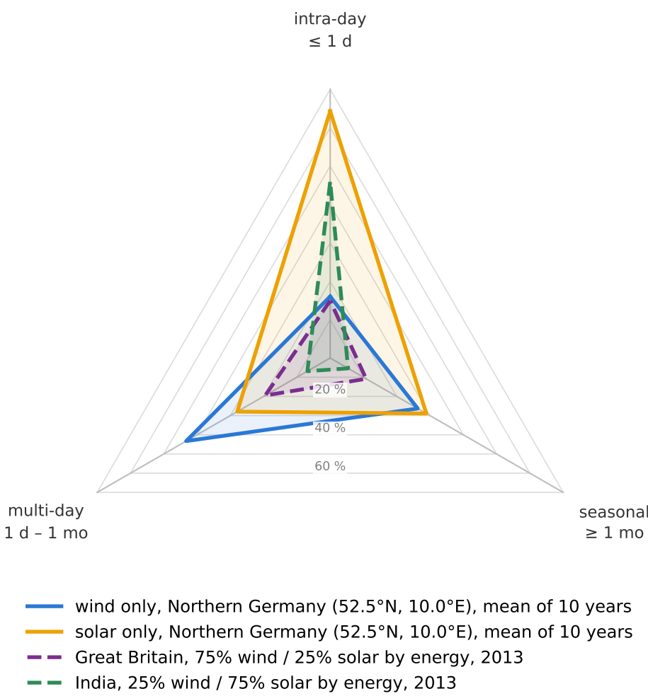
h Pure wind, pure solar and two countries supplied by a wind/solar superposition (dashed) energy cycled per period band, % of annual demand; countries from PyPSA-Earth country-aggregated profiles, 2013, total generation 1.2 × annual demand
