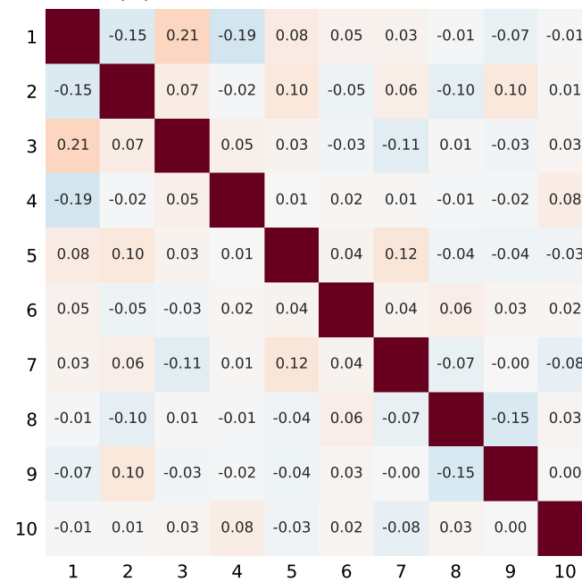
Pearson \rho , wind anomaly band worst |\rho| = 0.21 (limit 0.25)
