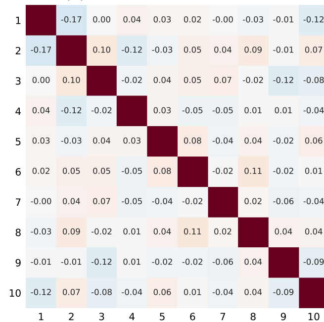
Pearson \rho , solar anomaly band worst |\rho| = 0.17 (limit 0.25)
