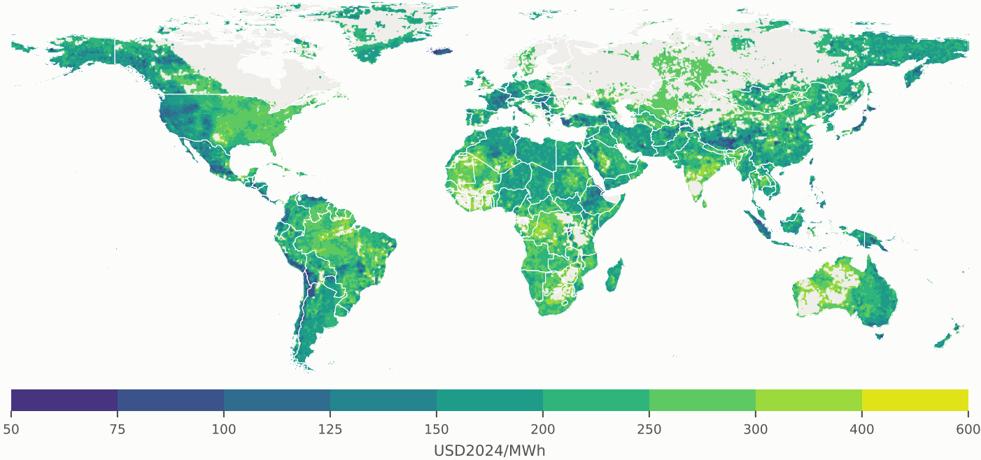
d LCOE (7% real WACC, 30 y, CF 85%, no grid connection)
