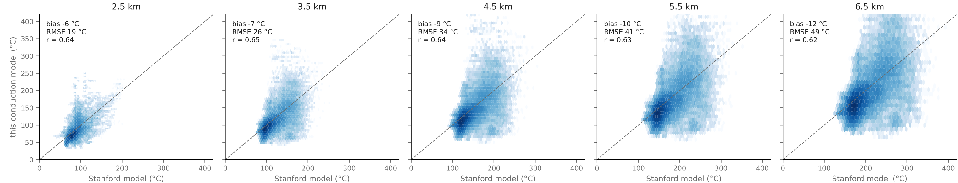
Rock temperature at depth, CONUS: 1-D conduction on Lucazeau heat flow vs the Stanford thermal model (n = 81,697 candidate areas)
