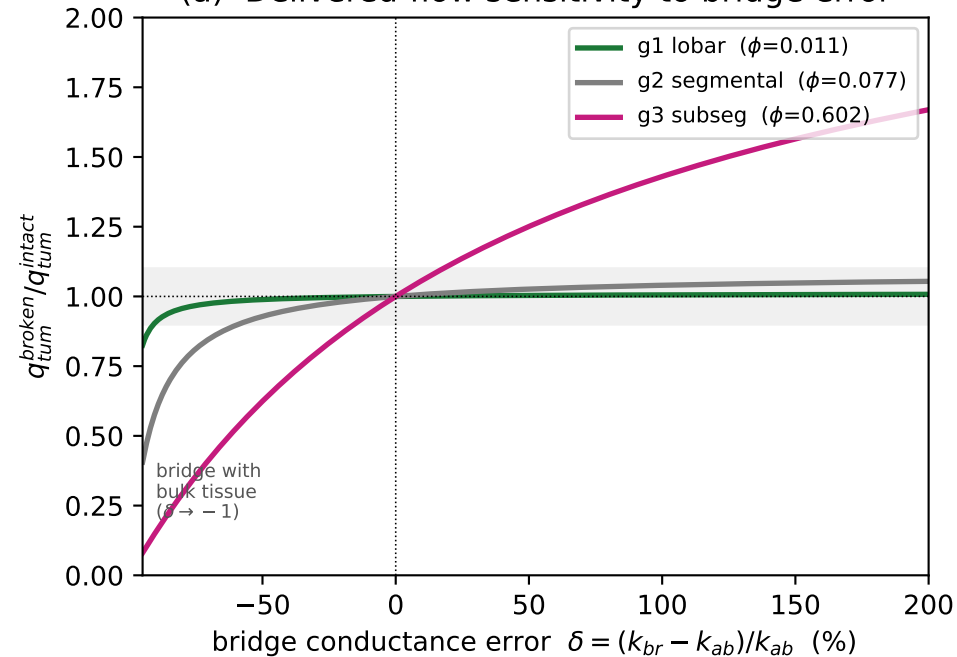
(a) Delivered-flow sensitivity to bridge error
