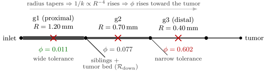
Figure 2: The three break locations of Table 1 on the delivery path (injection inlet, left, to tumor, right). Segment line width is drawn proportional to radius; the R^4 law in k_{ab} (6) means the resistance contributed by a break—and hence its resistance fraction \phi —rises steeply as the vessel narrows toward the tumor. A break in the wide proximal segment g1 ( \phi = 0.011 , green) barely perturbs delivered flow however it is bridged, whereas a break in the thin distal feeder g3 ( \phi = 0.602 , red) dominates the path resistance and demands an accurate bridge. The downstream siblings and tumor bed supply \mathcal{R}_{\text{down}} ; the segment upstream of the inlet supplies \mathcal{R}_{\text{up}} .
