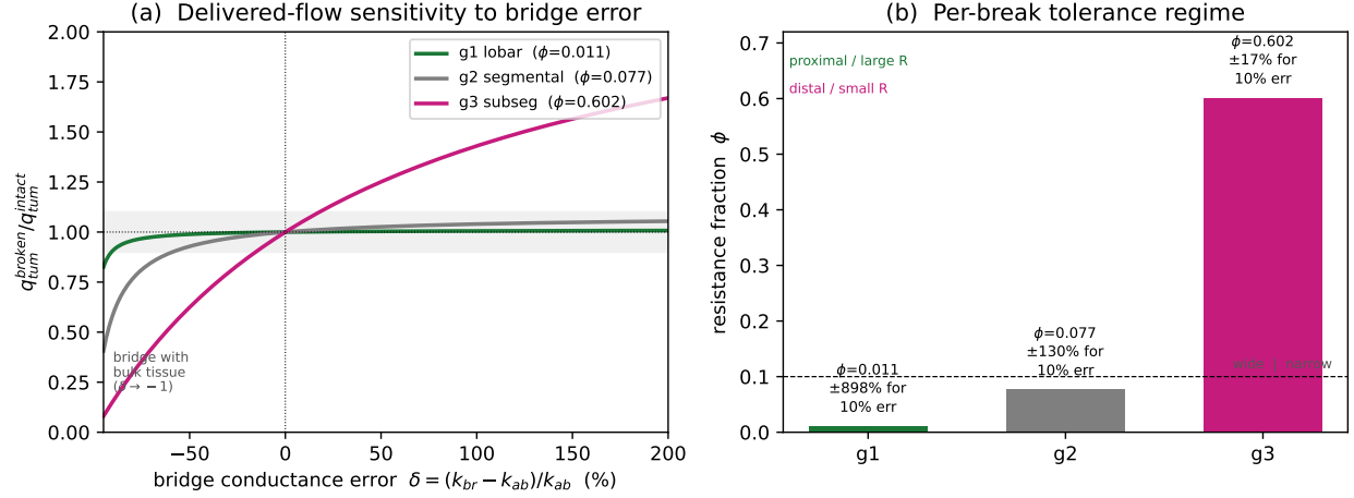
Figure 3: (a) Exact delivered-flow ratio versus bridge-conductance error \delta for a break in each generation; the shaded band marks a \pm 10\% flow tolerance. The proximal curve (g1) is nearly flat—delivered flow is almost independent of how the break is bridged—while the distal curve (g3) tracks \delta steeply. (b) The resistance fraction \phi by generation; annotations give the bridge error tolerated for a 10% flow error. Breaks with \phi below the dashed line lie in the wide-tolerance regime and may be bridged crudely; those above require accurate calibration of k_{br} to k_{ab} .
