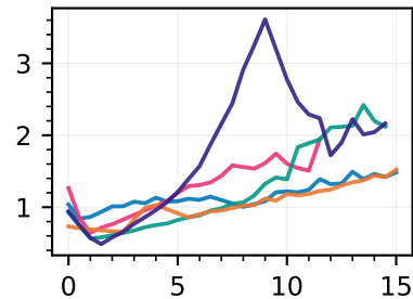
-Cp,min vs \alpha
