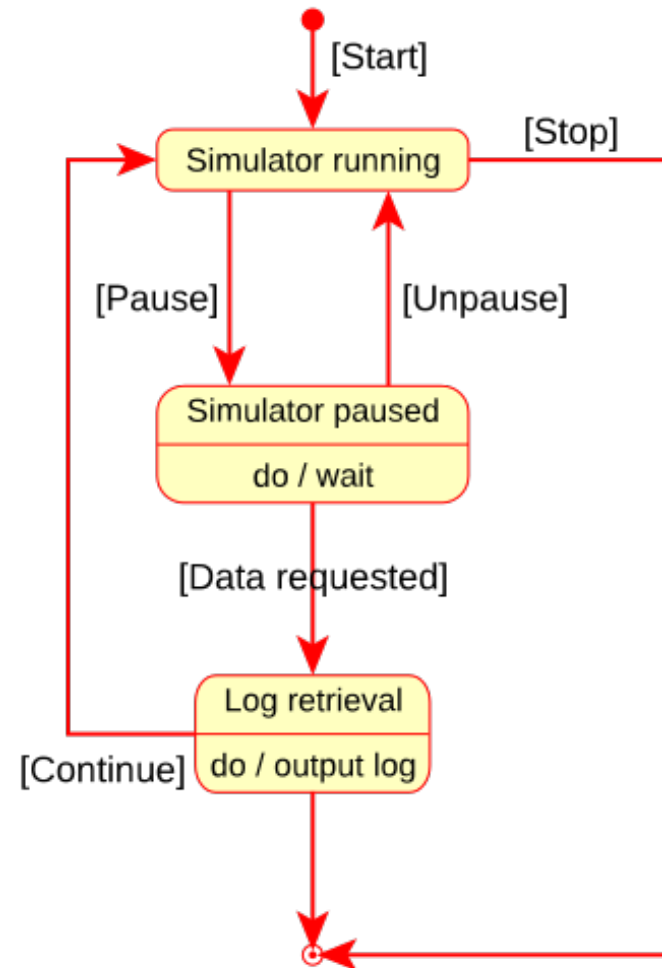
UML State Diagram example Source: Wikimedia
