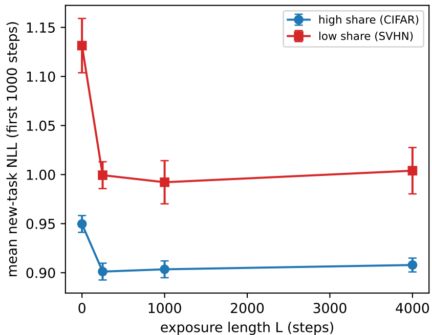
Adaptation window: NLL
