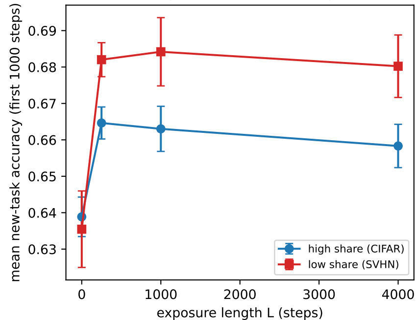
Adaptation window: accuracy
