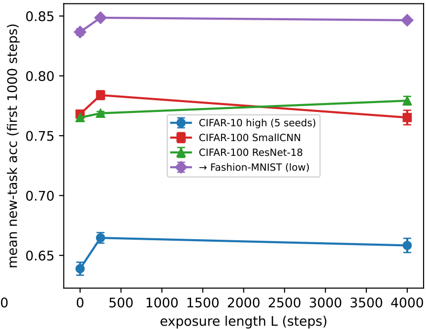
The window across benchmarks
