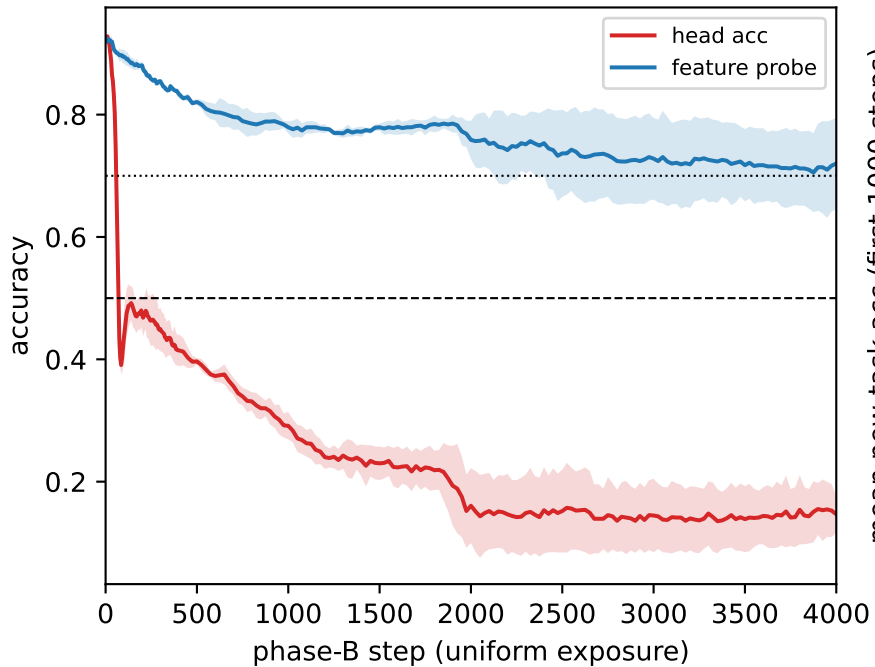
CIFAR-100 (25+25 classes), SmallCNN
