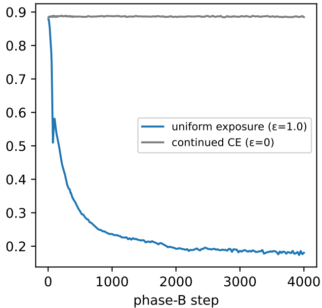
head accuracy
