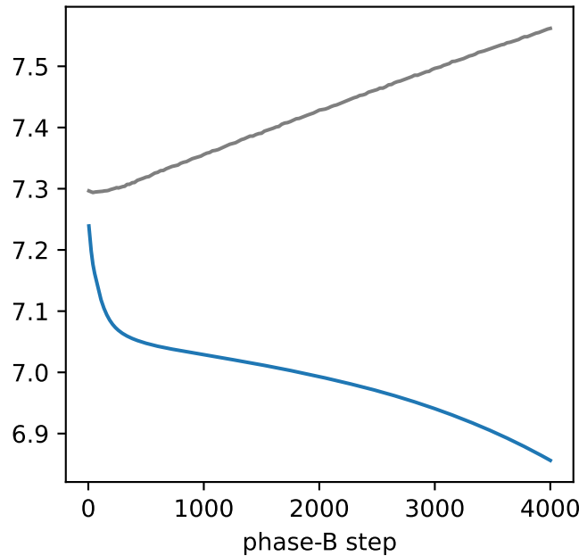
\|W_2\| (Frobenius)
