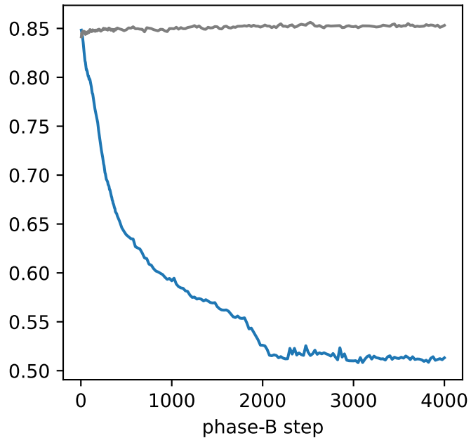
feature probe
