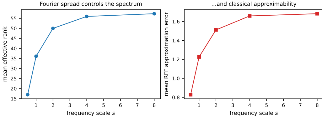
Figure 3: The frequency scale s of the high-dimensional feature map is the dominant design knob (exp04, depth 2). Left: s versus effective rank. Right: s versus RFF approximation error. Both follow s perfectly monotonically ( \rho = +1.000 ).
