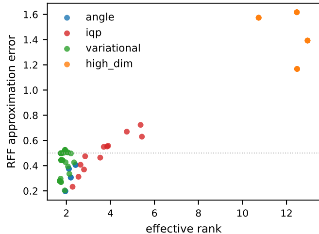
concentrated spectra are easier to simulate
