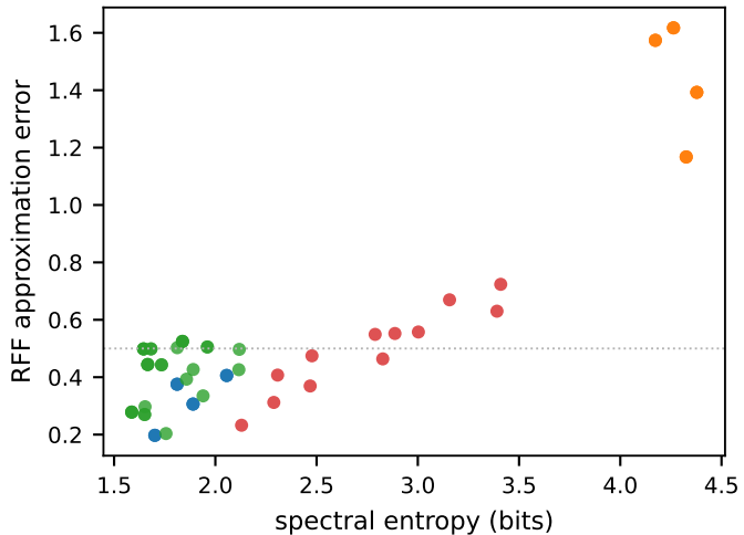
spectral entropy vs simulability
