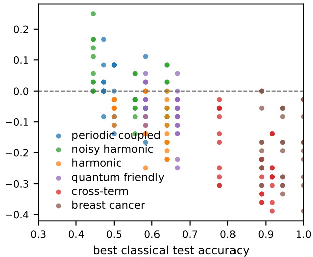
quantum advantage
