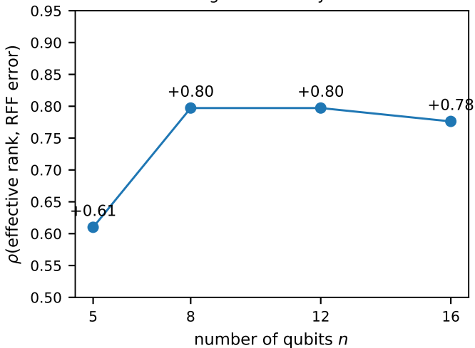
H1 strengthens with system size
