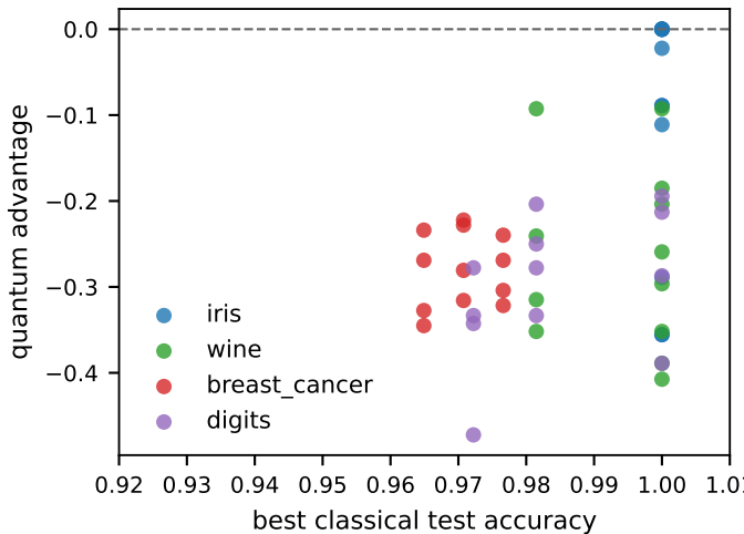
Real data: no advantage where classical saturates
