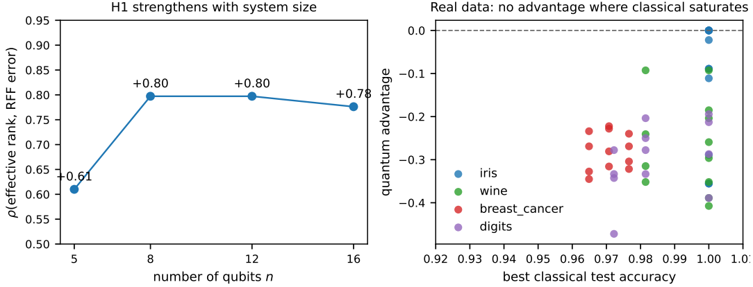
Figure 4: Scaling and real-data robustness. Left: the simulability relation ( \rho of effective rank vs. RFF error) strengthens with system size, from 5 to 16 qubits. Right: on four real datasets the classical baseline is near-saturated and quantum advantage is never positive.
