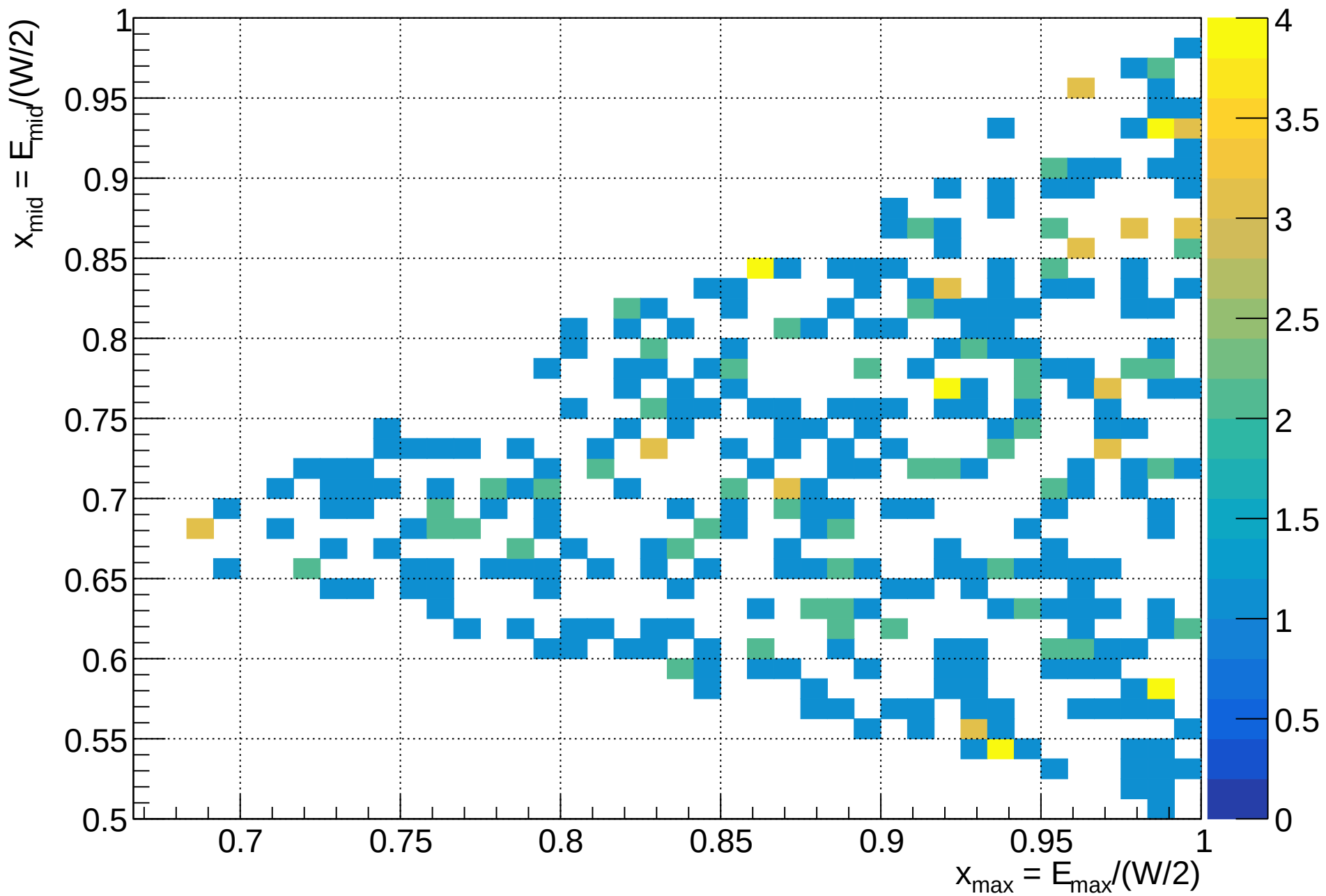
Three-photon Dalitz plot (Ore-Powell generator)
