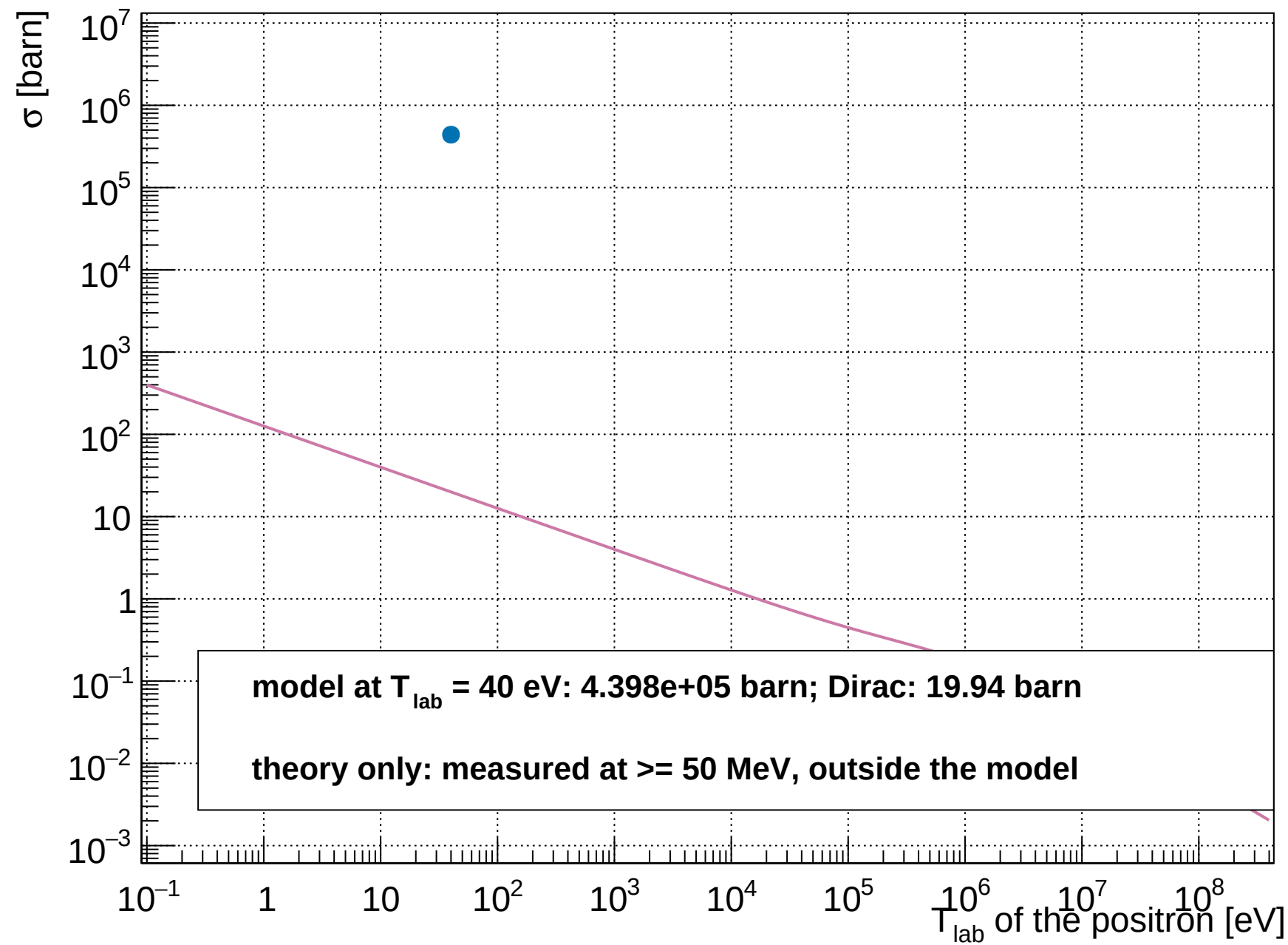
Annihilation in flight (Dirac, QED) vs the model's barrier cross section
