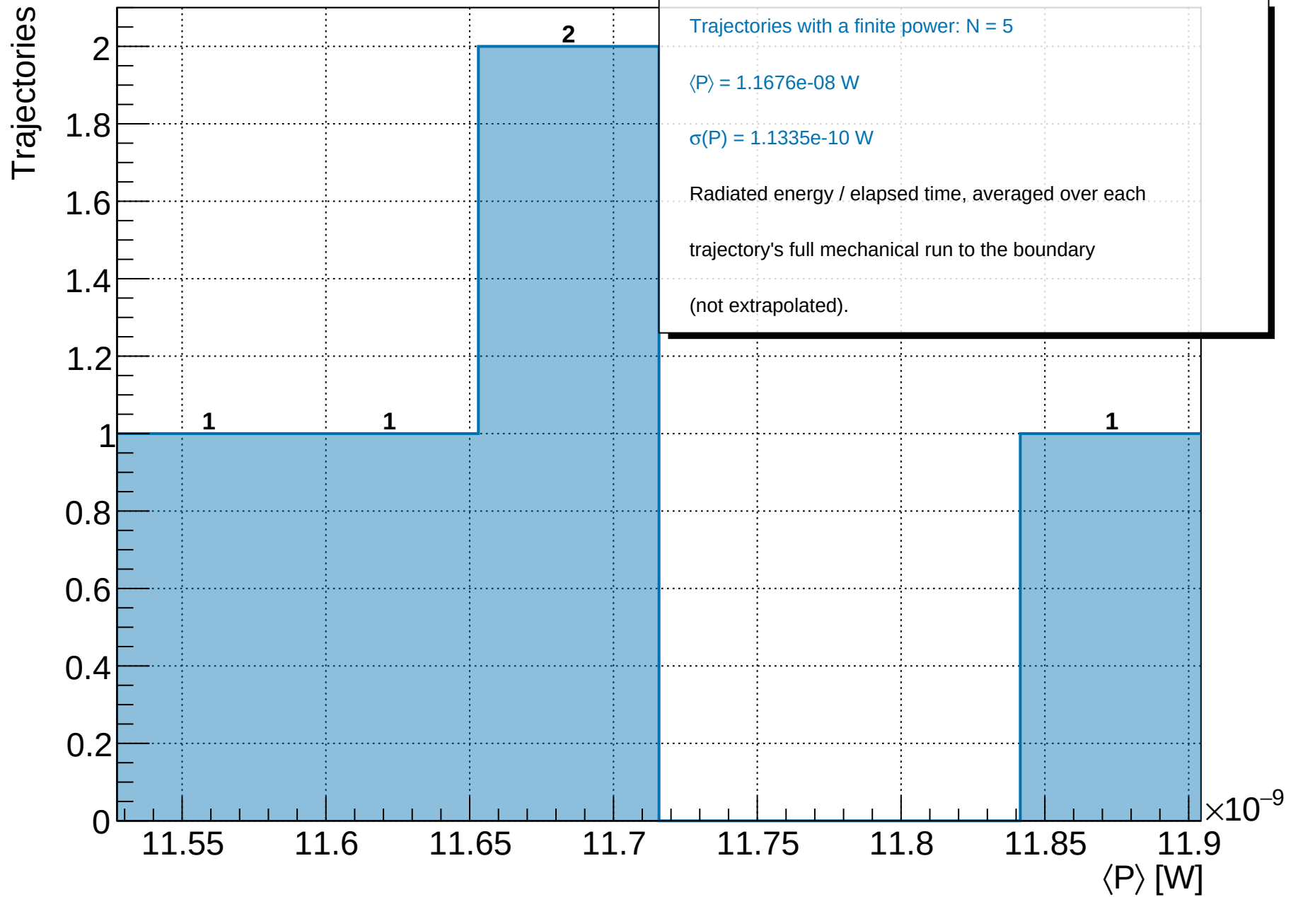
Orbit-averaged radiated power of the CREM collapse
