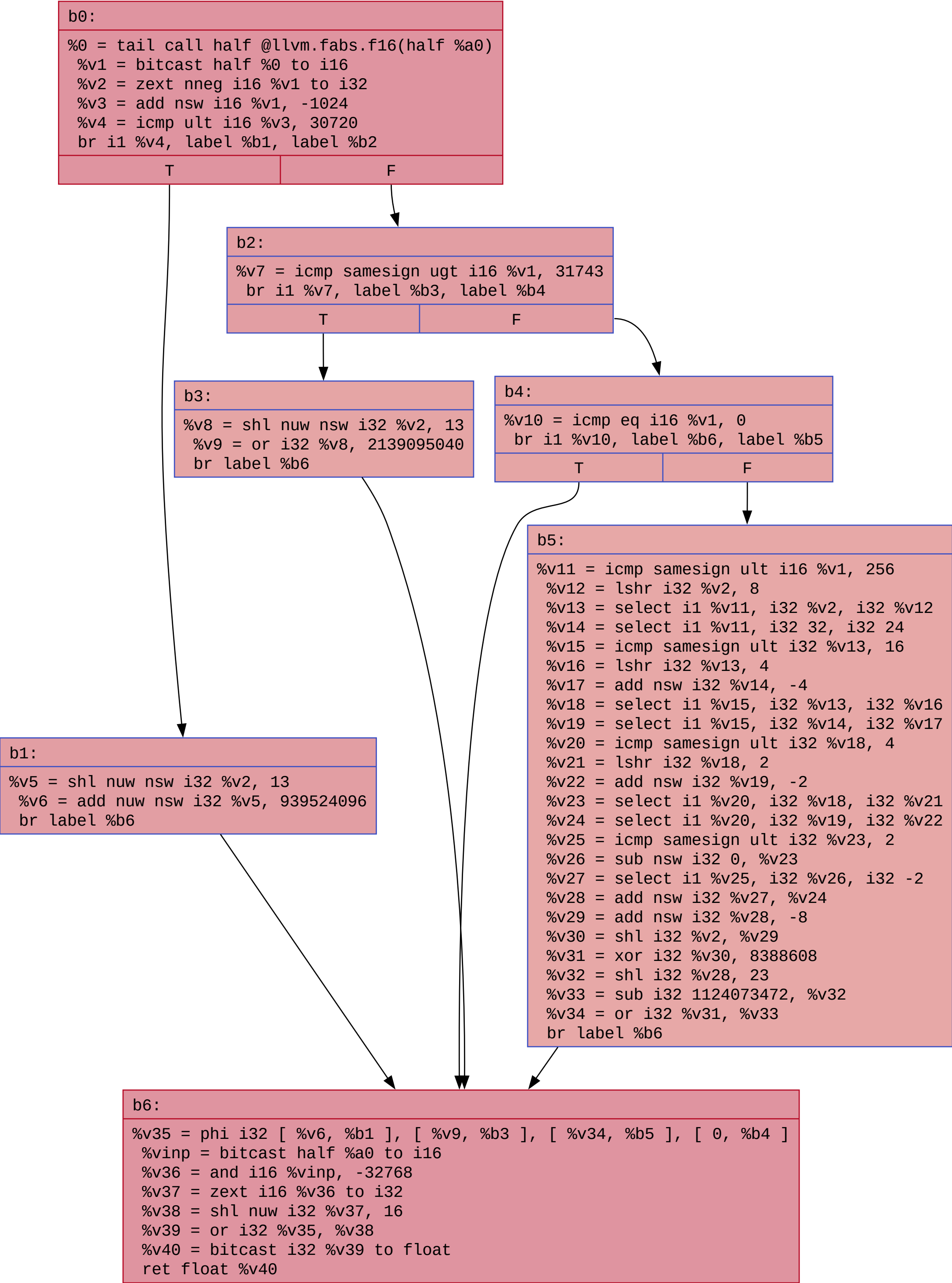
CFG for '__extendhfsf2' function
