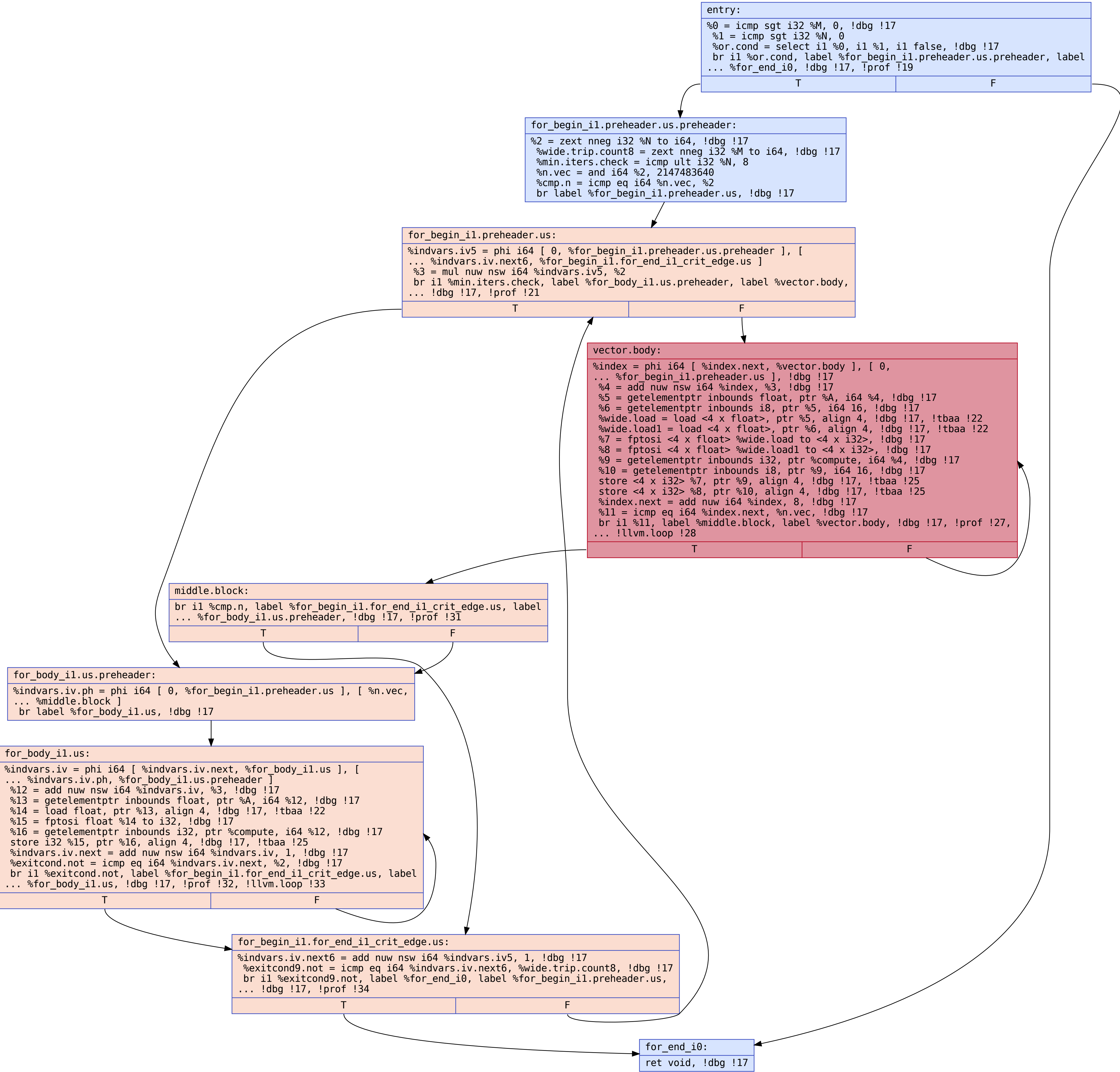
CFG for 'cast_compute_' function
