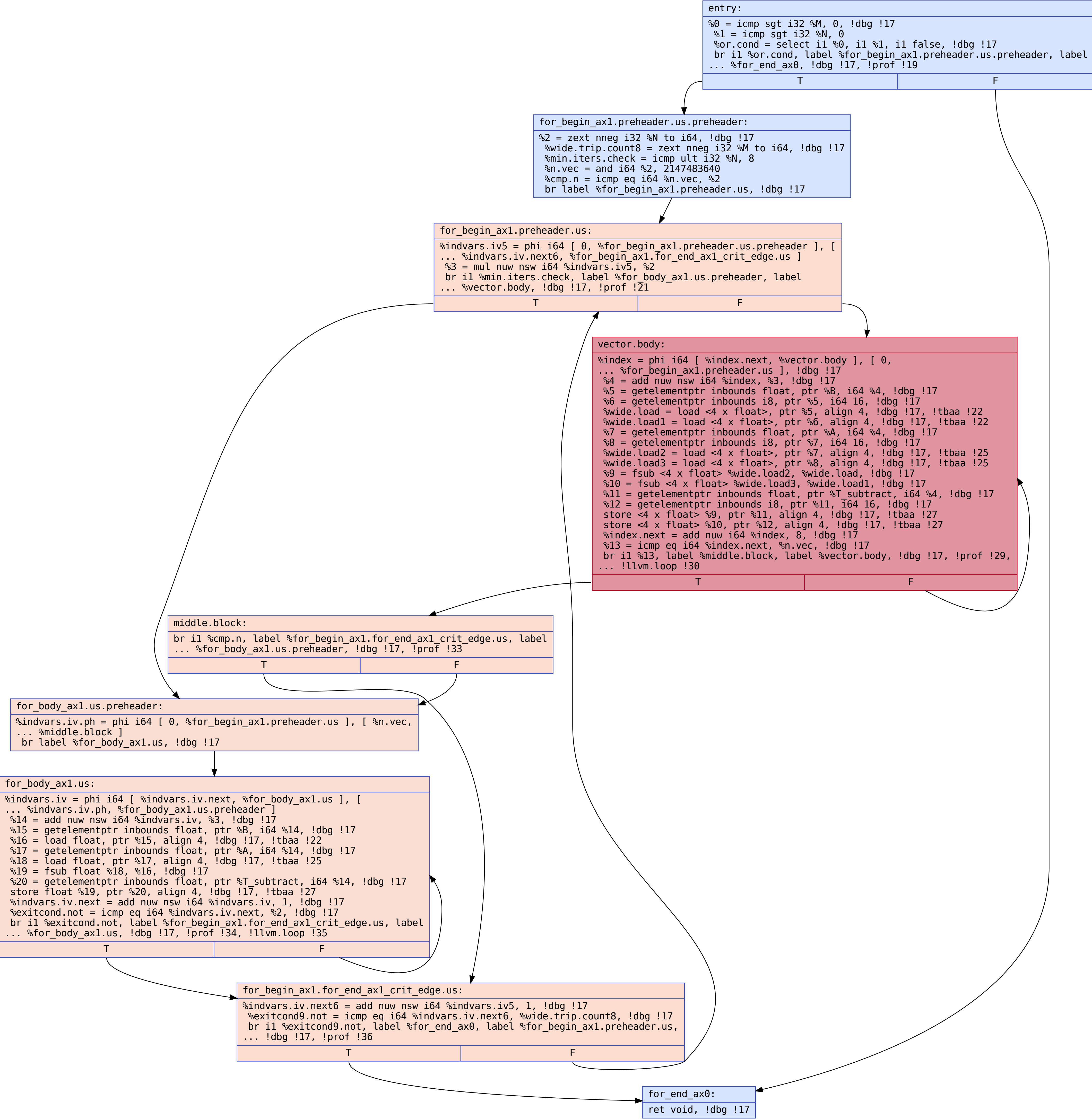
CFG for 'sub_compute_' function
