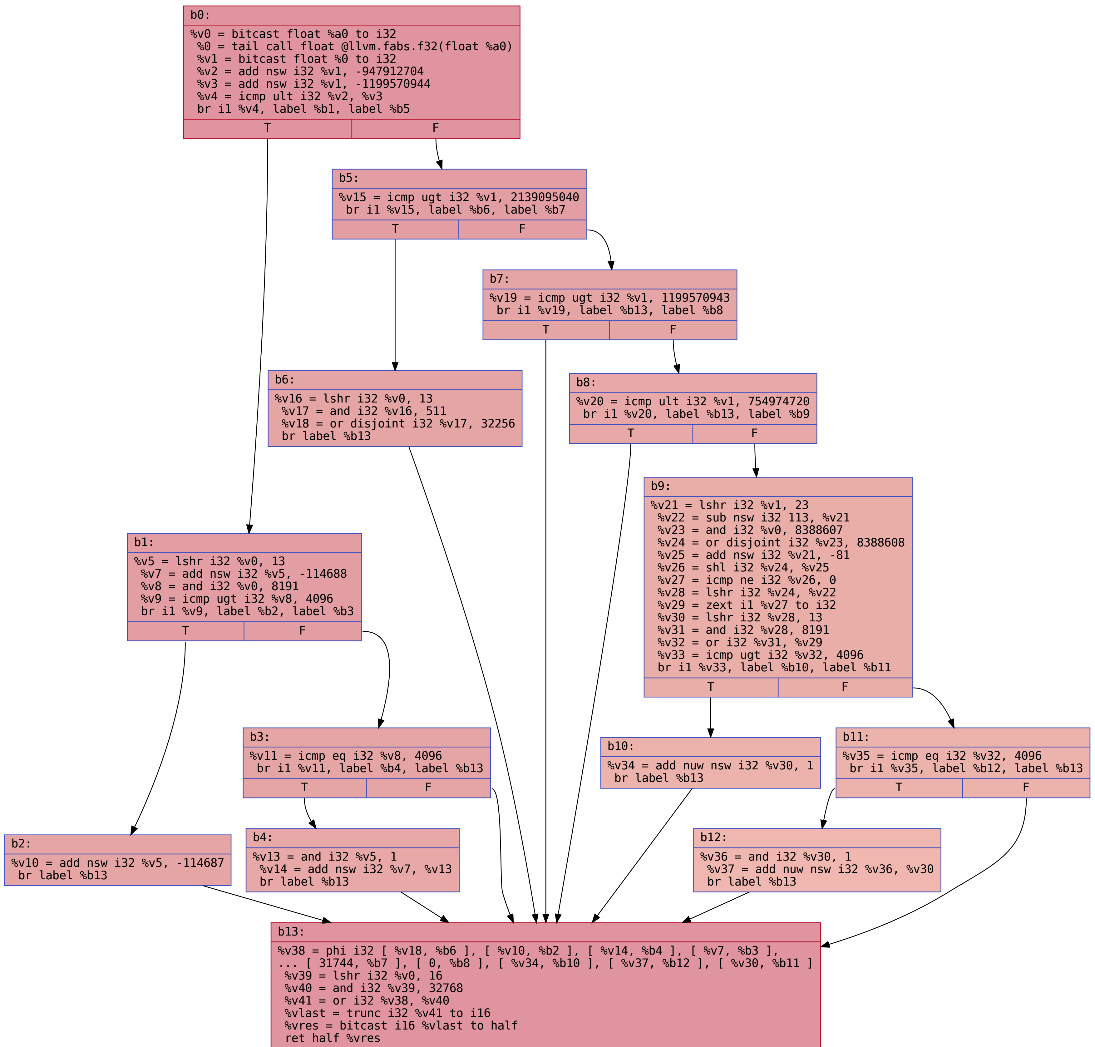
CFG for '__truncsfhf2' function
