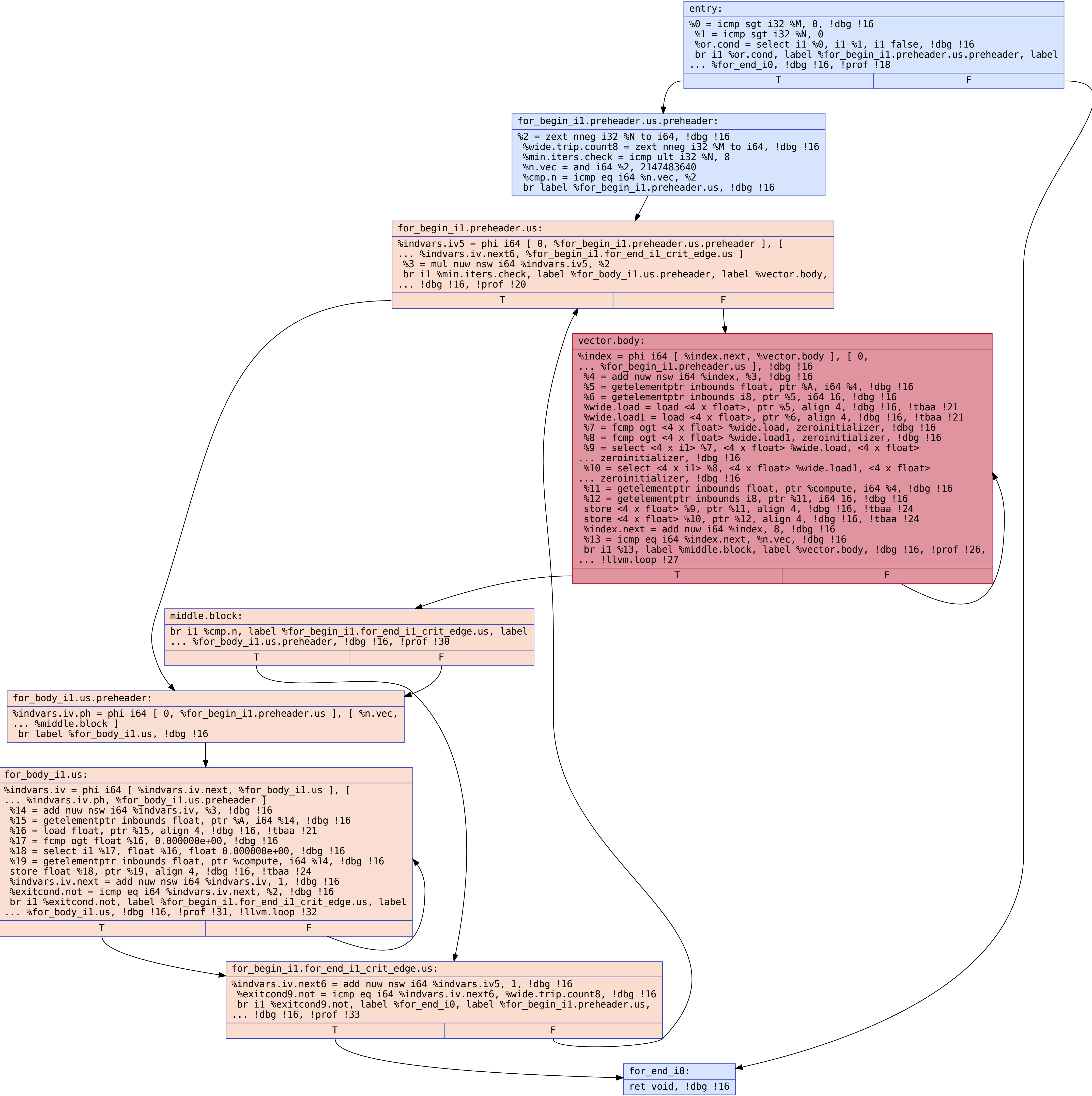
CFG for 'relu_compute_' function
