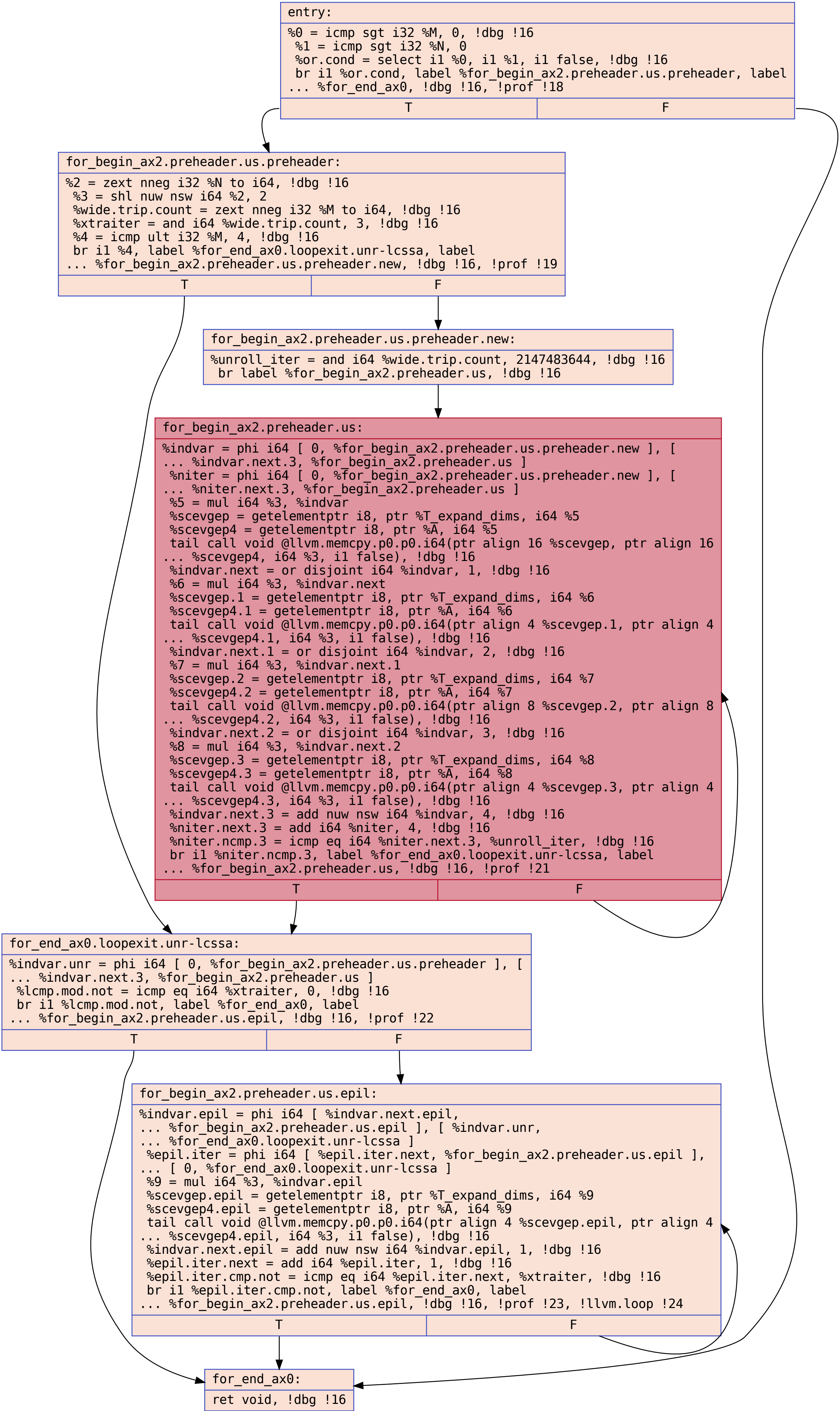
CFG for 'unsqueeze_compute_' function
