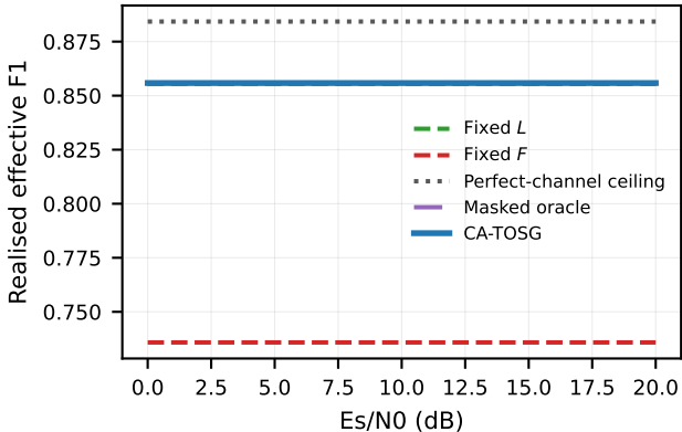
RAYLEIGH, validate, B_{\max} = 0.20
