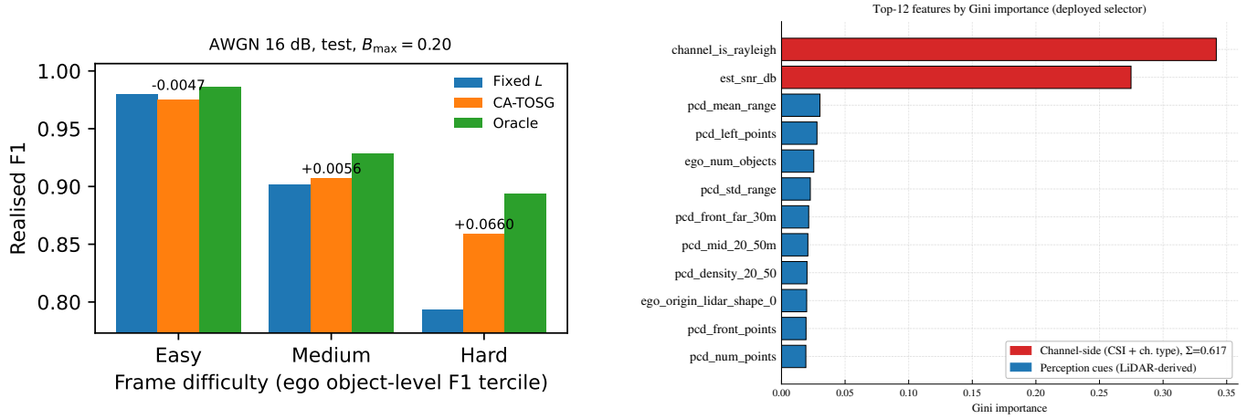
Fig. 3. Left: realised F1 by frame-difficulty tercile (ego object-level F1) on OPV2V test at B_{\max} = 0.20 at a single reliable-channel grid point (AWGN 16 dB) with the frozen selector; numbers above bars are CA-TOSG–Fixed- L , the hard-frame gain being +0.0660 (95% CI [+0.0591, +0.0730]). Right: top-12 features by Gini importance of the frozen B_{\max} = 0.20 selector—the channel-side features jointly account for 61.7%, the 21 perception-side cues for the remaining 38.3%, none above 3.0% alone. Importance is not sufficiency (the ablation section of the main paper).
