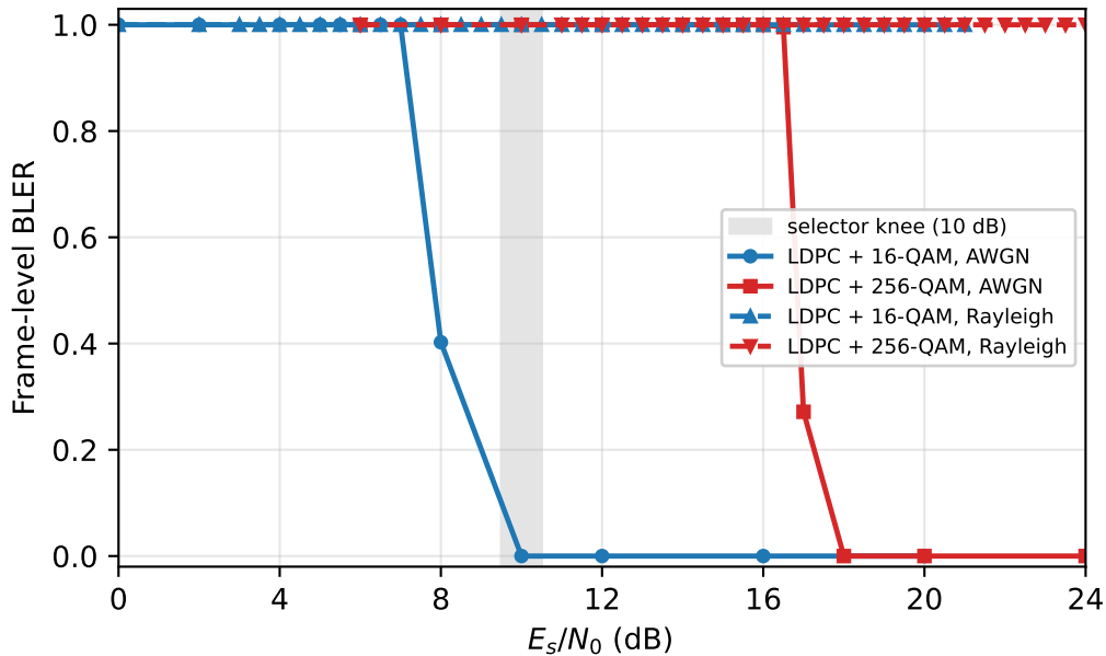
Frame-level BLER: LDPC + QAM over AWGN and Rayleigh
