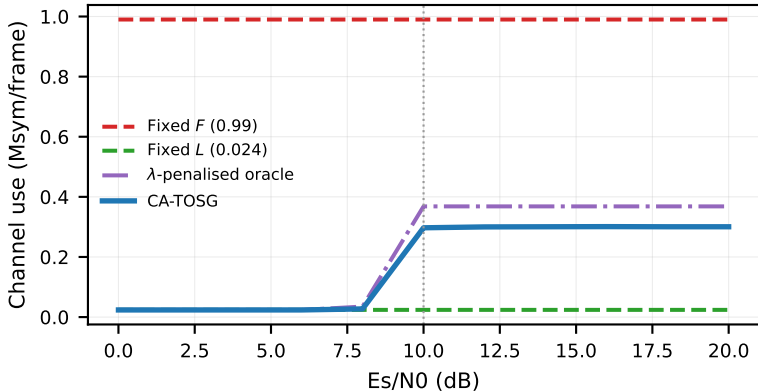
AWGN, validate, B_{\max} = 0.20
