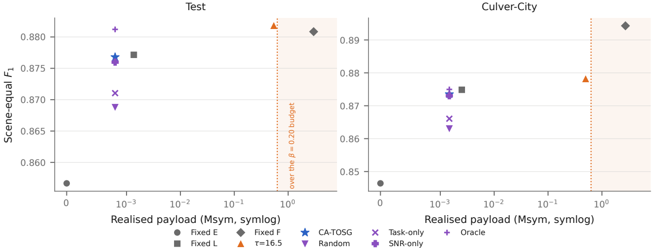
Fig. 2. Scene-equal F_1 against realised payload on each held-out split. Both quantities are shown together, because ranking on either alone misrepresents the trade-off: the arms differ by more than three orders of magnitude in payload—at least 1,090\times between the cheapest and the dearest transmitting arm on either split—and by hundredths in F_1 . The dotted line is the \beta = 0.20 ceiling and the shaded region is over budget, so Fixed F is visibly not a competitor at the primary budget. The x axis is symlog rather than logarithmic: Fixed E spends exactly zero, which a logarithmic axis cannot show. Random, Task-only, SNR-only and Oracle are the matched-payload policies of Table IV and sit at CA-TOSG’s own payload; Oracle is not deployable.
