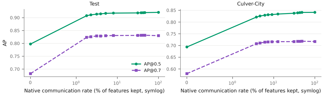
Fig. 7. Where2comm on its native communication-rate axis. The horizontal axis is the fraction of features retained, not a bit budget.
