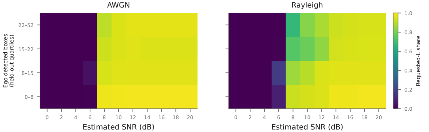
Fig. 5. Where the frozen policy requests object-level cooperation, pooled over both held-out splits. Colour is the requested-action share of L; frames without an available collaborator are structurally executed as E and are counted here by what was requested, never by what was executed. The horizontal axis is the 11 protocol SNR grid points and the vertical axis is the ego detected box count in quartiles of the pooled held-out rows, both fixed before plotting; cells are drawn without smoothing or interpolation, so no structure is shown between points that were evaluated.
