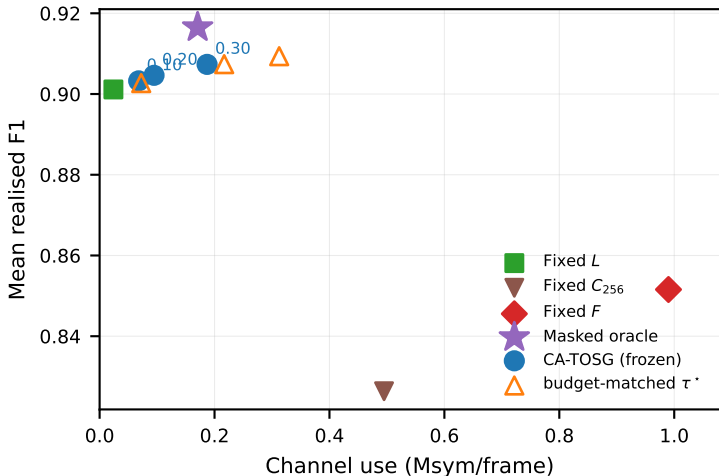
OPV2V test, frozen replay (200 realisations)
