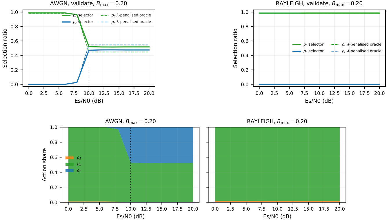
Fig. 4. Per-mode selection ratios versus SNR on OPV2V validate at B_{\max} = 0.20 , from the frozen grid. Top: the frozen selector (solid) against that budget's \lambda -penalised oracle (dashed) — the oracle sees the frame BLER, not the per-frame block outcome, so it is not clairvoyant. Bottom: stacked-area view of the selector's action distribution over the deployed action set \mathcal{S} = \{E, L, F\} under AWGN and Rayleigh (the dominated C_{256} is a physical-layer comparator, not a deployed action, Section III-B); the dotted line marks the measured 10 dB policy knee. Two readings: under AWGN \rho_F steps from 0 to 0.472 at 10 dB and is flat above it, and under Rayleigh the selector's \rho_E is 0.002 (test) / 0.000 (Culver-City) while the oracle spends \rho_E = 0.157 / 0.133 there — the E -collapse limitation of Section VI-G. The three-budget version is the per-budget action distributions (repository figure product).
