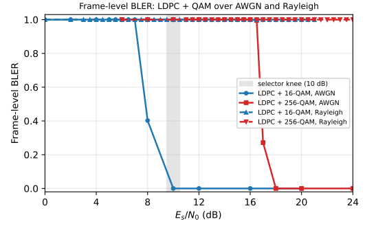
Fig. 2. Block-error rate of the feature-level message under LDPC 1/2 with 16-QAM and 256-QAM, over AWGN (solid) and Rayleigh (dashed) channels. The 16-QAM AWGN cliff (an 8–12 dB transition, onset 8.0 dB) defines the selector knee (shaded); the 256-QAM cliff sits far to its right (onset 16.5 dB), so by the time 256-QAM is reliable the 16-QAM block is already error-free. Under Rayleigh fading both curves degrade so slowly that, under the all-or-nothing frame model evaluated here, feature-level transmission never becomes reliable in 0–20 dB, explaining the selector’s conservative L -only behaviour.
